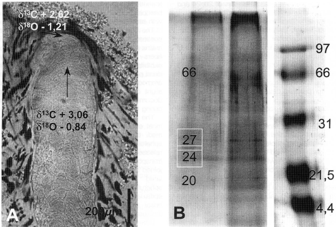
Figure 7. Spirastrella (Acanthochaetetes) wellsii , a chaetetid coralline sponge. a. The uppermost growing zone of Acanthochaetetes (top of a tube wall) with stable isotope values from different growth zones. b. SDS gel showing four detected macromolecules (20 kD, 24 kD, 27 kD, and 66 kD). The standard ladder on the right is for comparison of molecule size.
