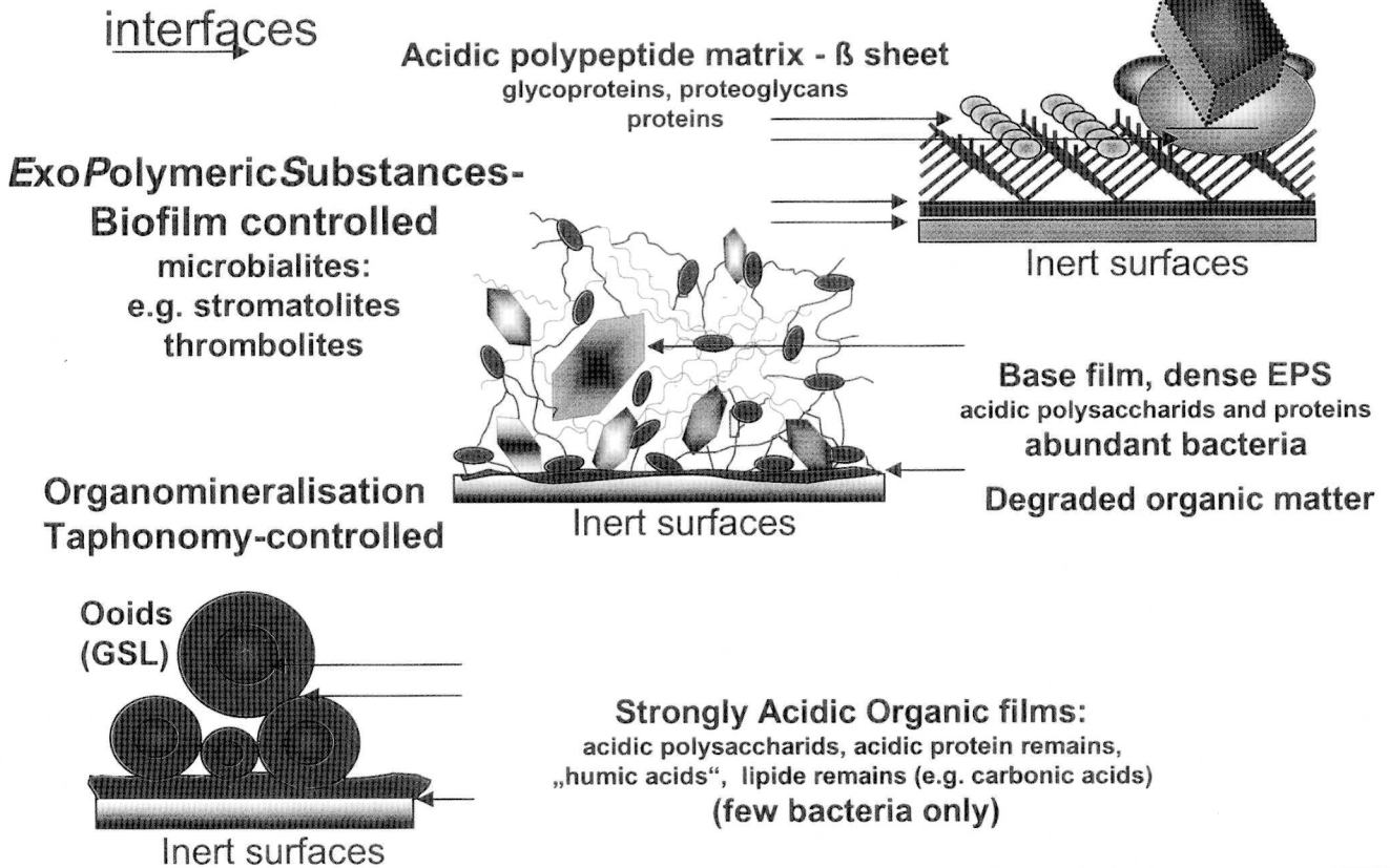
Figure 1. Model for evolution of biomineralization from organomineralization (taphonomy-controlled) of Great Salt lake Ooids via an exo-polymeric substance (EPS) to a biofilm-controlled calcification in microbialites to matrix-mediated mineralization of coralline sponges.
