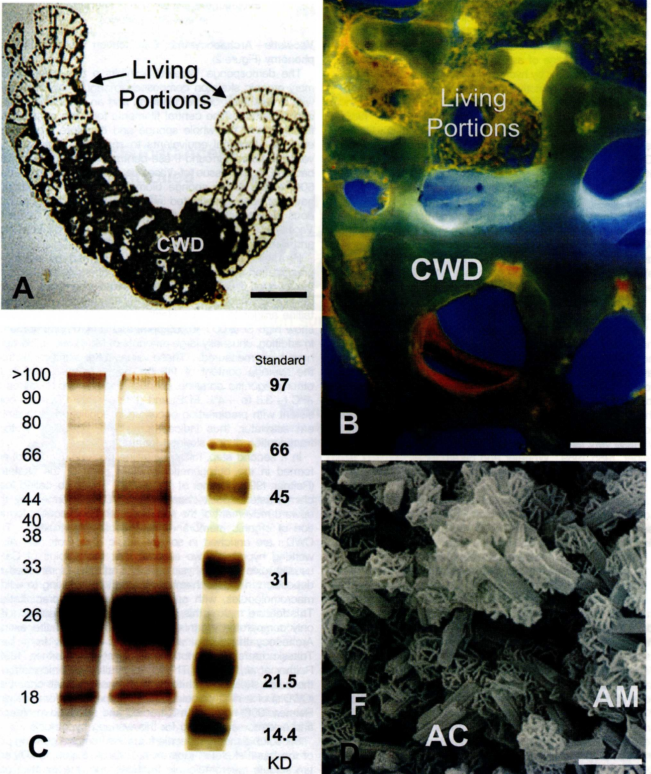
Figure 2. Vaceletia —a modern archaeocyathid sponge. a. Vaceletia n.sp. of the branching type, from Osprey reef. Living and dead portions. b. Tetracycline stained waste chambers. c. SDS PAGE of waste chamber organic mucus with 10 different macromolecules (indicated on the left). d. SEM micrograph of newly formed aragonite crystals in calcium waste chambers (CWD).
