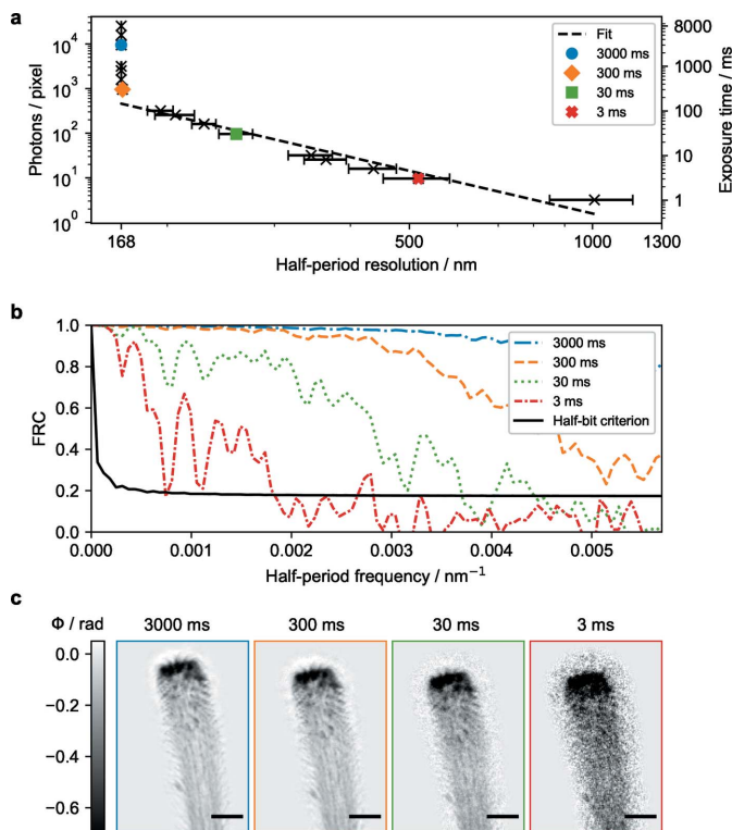
Figure 5 (a) Half-period resolution of holographic reconstructions (2D projections) as a function of the number of photons per pixel. (b) Estimation of the half-period resolution via the FRC for different exposure times. (c) Phase reconstructions of a spider attachment hair for different exposure times ranging from 3 to 3000 ms. At 300 ms, the detector sampling limits the achievable resolution. The scale bar indicates 5 \mu\text{m} .
