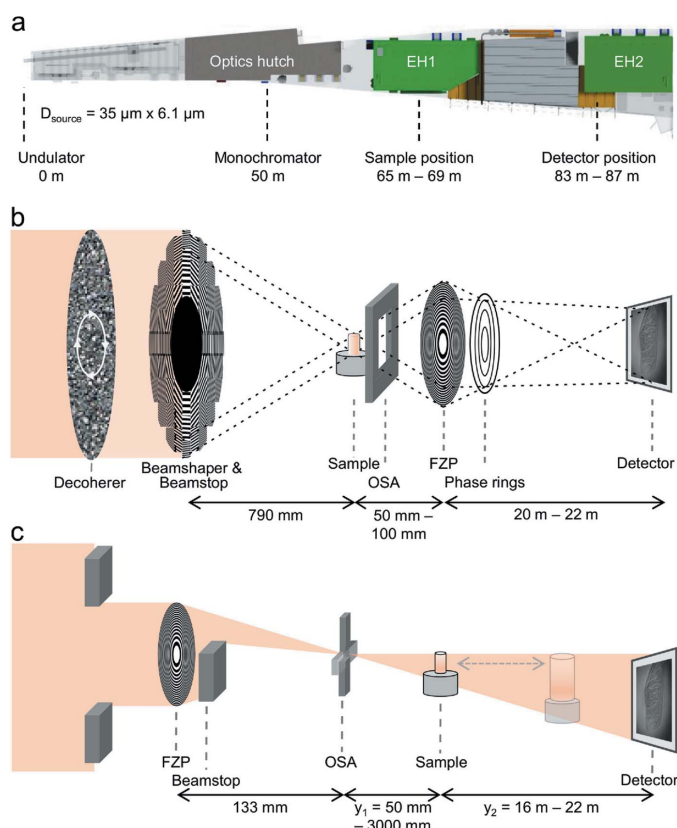
Figure 1 (a) Overview of the beamline P05 with relevant hardware components and their distances to the source. The nanotomography setup is located in the first experimental hutch (EH1) while the camera is placed in the second experimental hutch (EH2). (b) Zernike phase contrast implemented in a standard transmission X-ray microscope and (c) near-field holography setup using a Fresnel zone plate (FZP) as focusing optics. This setup was also used for the near-field ptychography measurements.
