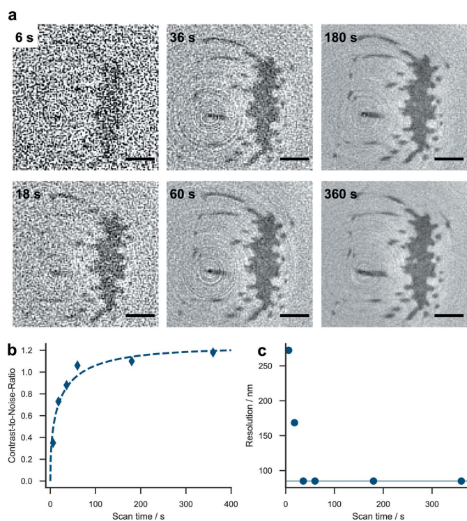
Figure 3 Fast Zernike phase contrast tomography with a photon-counting detector. (a) Reconstructed slices of a spider attachment hair with different scan times. (b) CNR for the different scan times. For details of the fit, refer to Flenner et al. (2020c). A high CNR is already reached after 60 s. (c) Half-period resolution as calculated from the FRC. The effective pixel size (85 nm, solid horizontal line) limits the resolution after 36 s scan time. The scale bar indicates 2 \mu m.
