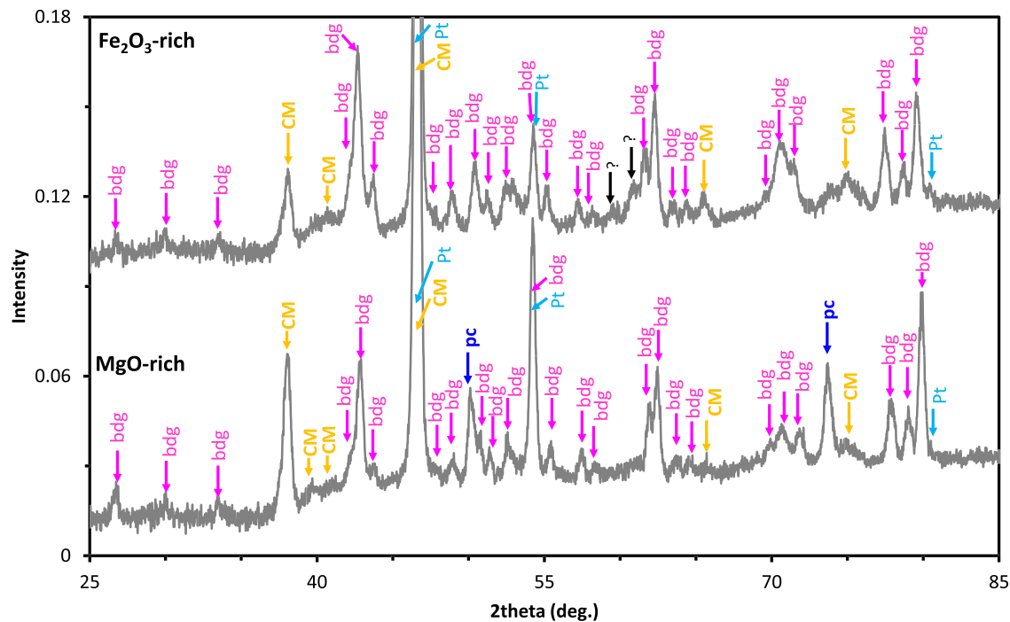
Figure 2. Representative X-ray diffraction spectra of run products (Run I567). (top) Fe 2 O 3 -rich sample. (bottom) MgO-rich sample. Bridgmanite (bdg), CaMn 2 O 4 -type MgFe 2 O 4 (CM), and (Mg,Fe)O-periclase (pc) phases were identified, as well as the Pt from the sample capsules.
