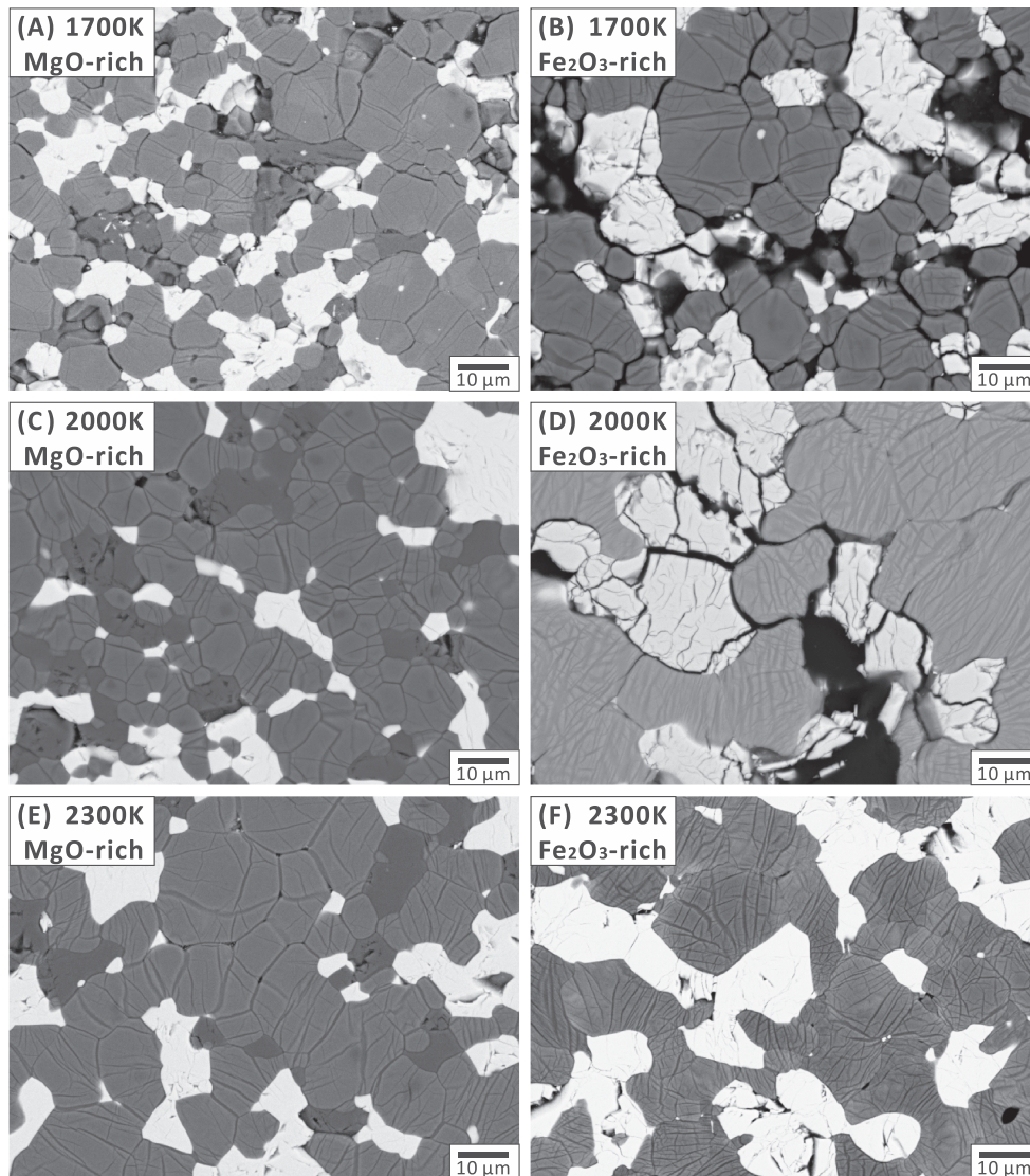
Figure 1. Backscattered SEM images of run products at 27 GPa and 1700–2300 K for both (a, c, and e) MgO-rich and (b, d, and f) Fe 2 O 3 -rich samples, which appear as coexisting bridgmanite (gray) + MgFe 2 O 4 (bright) + (Mg,Fe)O (dark) phases and bridgmanite (gray) + MgFe 2 O 4 (bright) phases, respectively.
