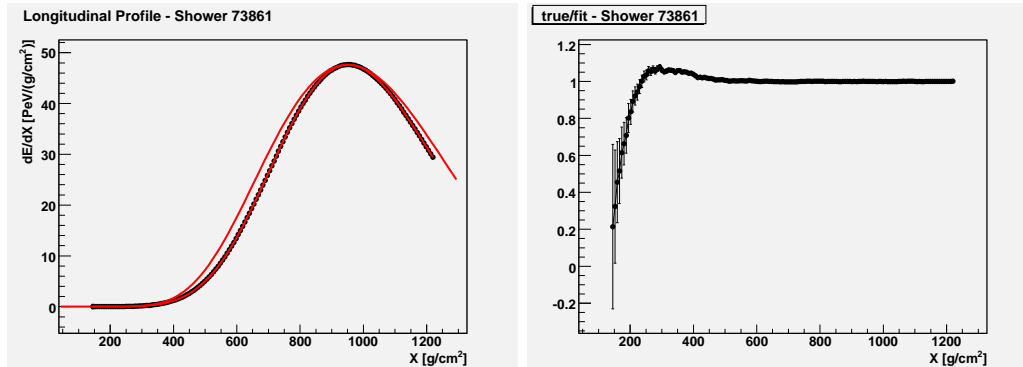
Figure 6.2: Left: longitudinal profile (energy deposit as a function of slant depth) for a simulated shower induced by a photon at 10^{19} eV. Black dots for the data points, dashed red line for CORSIKA 6-parameters GH fit, thick red line for the 4-parameters GH fit. Right residuals from the 4-parameters fit.
