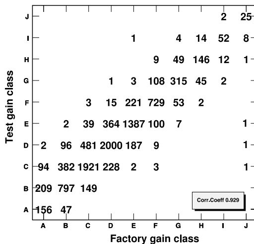
Figure 4.13: Left: table of the gain class definitions. Right: distribution of the PMTs in the corresponding gain classes, the acceptance test results versus the factory results.
