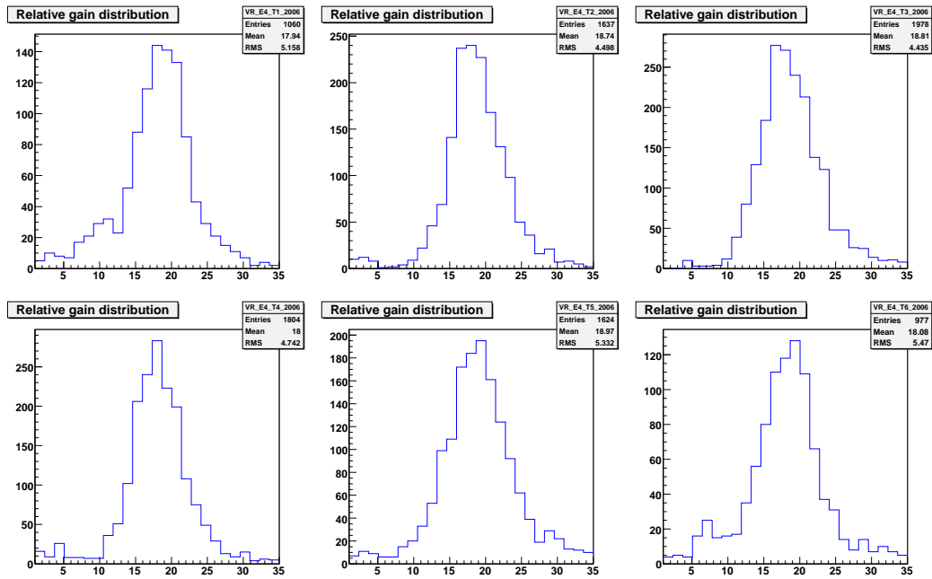
Figure 5.14: Real data: relative gain distributions for the 6 telescopes in Los Morados, collected data since Feb 2006. In order to correctly calculate the normal to virtual gain ratio, events with a single triggered pixel per virtual channel have been used for this analysis and a cut on minimum signal charge has been applied.
