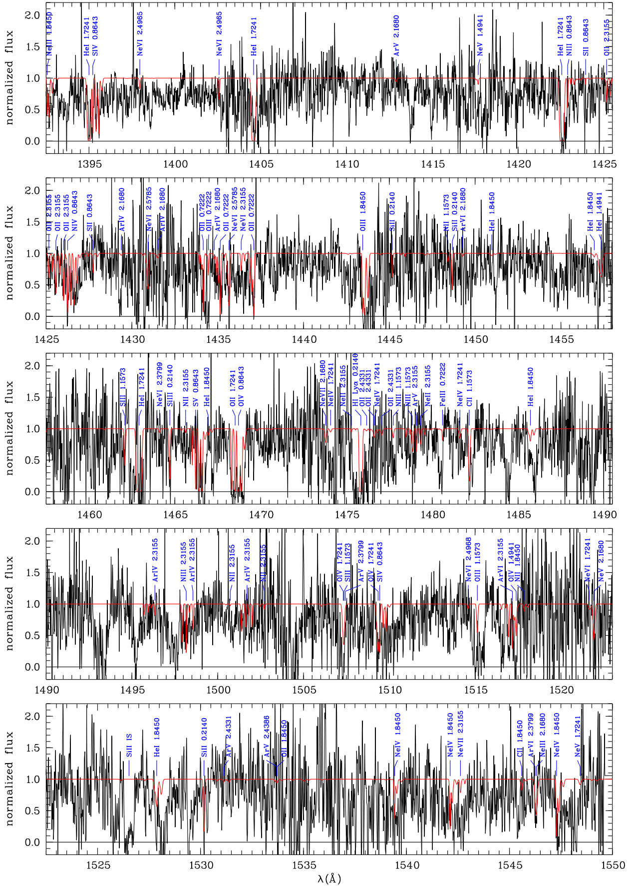
Fig. 4.24: Predicted metal line spectrum in the range 1393 – 1550 Å in comparison to the normalized STIS data (see text for details).
