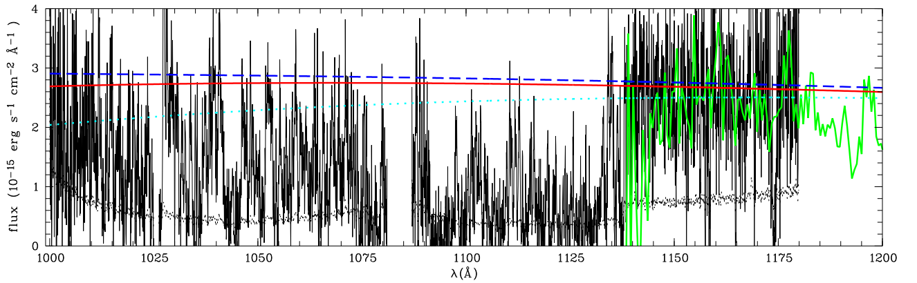
Fig. 5.1: The FUSE data and the extrapolated continuum. The solid line presents the continuum considering the Cardelli et al. (1989) extinction curve and E(B-V) = 0.025 (Schlegel et al. 1998). For comparison we show the extrapolated continuum using E(B-V) = 0.060 adopted from X-ray observations (Reimers et al. 1995) and the Cardelli et al. (1989, dotted line) or the Pei (1992, dashed line) extinction curve, respectively. Furthermore, we overlay the low resolution STIS data.
