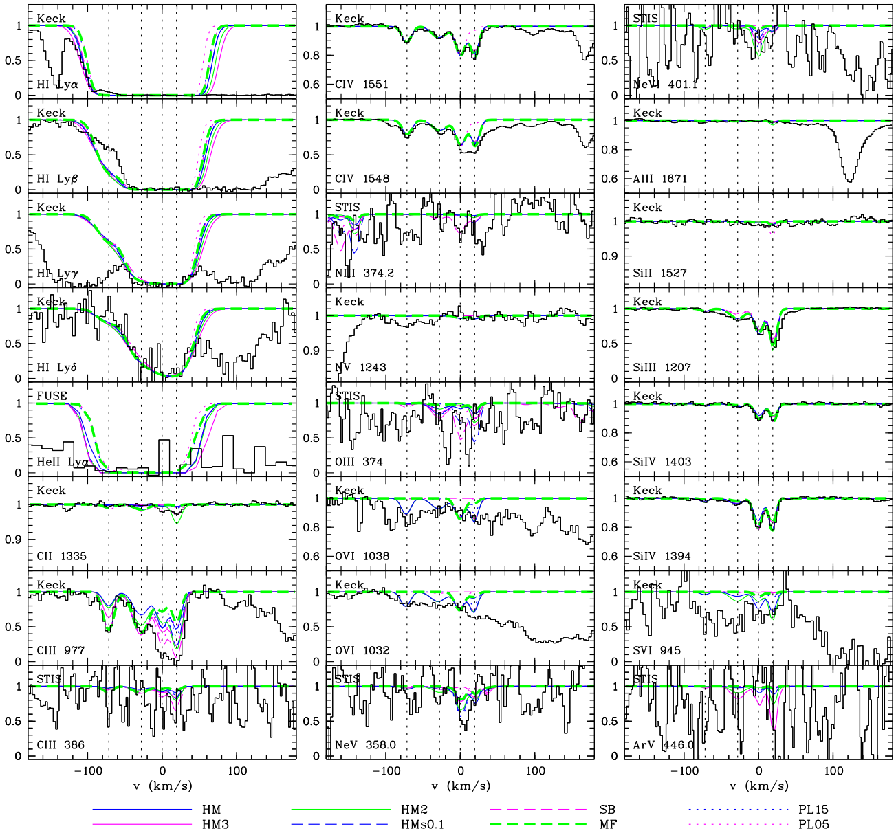
Fig. 4.17: Observed and modelled absorption lines of the system at z = 2.4386 . The preferred model is MF.
