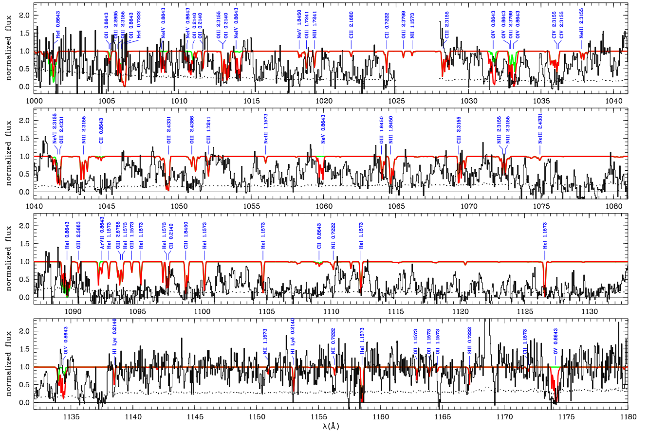
Fig. 5.3: Predicted metal line spectrum in comparison to the data. The predicted features are identified given the ion and the redshift of the system where they arise.
