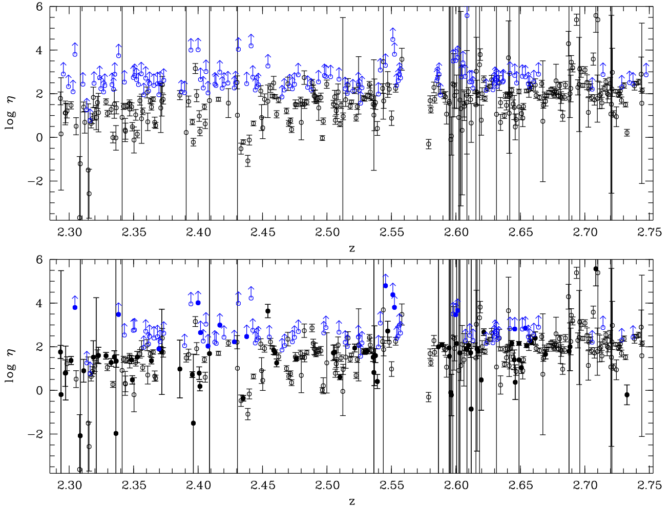
Fig. 5.4: Comparison of the \eta(z) distribution ignoring metal line and galactic \text{H}_2 absorption (upper panel) and taking them into account (lower panel). Absorbers affected by extra absorption are marked as filled circles. Lower limits are based on He II features without detected H I counterparts. Their Doppler parameters are chosen to be b = 27.0 \text{ km s}^{-1} .
