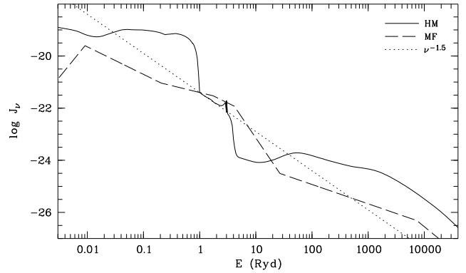
Fig. 2.1: The spectral shape of several radiation fields. The solid line represents the UV background of Haardt & Madau (2001, HM) at z \approx 3 , the long-dashed line shows the AGN-like spectral energy distribution derived by Mathews & Ferland (1987, MF), and the dotted line indicates the simple power law J_\nu \propto \nu^{-1.5} .
