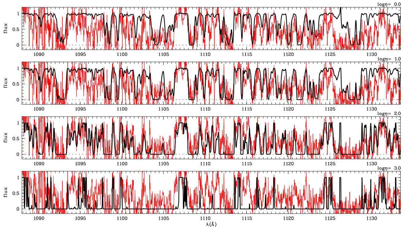
Fig. 6.1: Comparison of the observed He II data towards HE 2347-4342 to the metal subtracted, convolved H I spectrum scaled by \log \eta = 0.0, 1.0, 2.0, and 3.0 . Apparently, there are regions modelled well by \log \eta \approx 1.0 (e.g. 1112 - 1117 \text{ \AA} ) or \log \eta \approx 2.0 (e.g. 1096 - 1103 \text{ \AA} and \sim 1125 \text{ \AA} ), respectively, while \log \eta \approx 3.0 would lead only to sparse regions with non-zero UV flux, which is inconsistent with the observations in this redshift range. Features that appear nearly overestimated by \log \eta = 0.0 (at \sim 1104 \text{ \AA} , 1108.5 \text{ \AA} , and 1121.5 \text{ \AA} ) correspond to weak metal line systems (see text).
