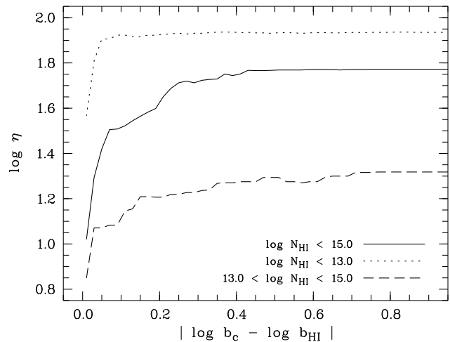
Fig. 6.9: Cumulative distribution of the median \log \eta with the distance d = |\log b_c - \log b_{\text{HI}}| from the b(N) cut-off. The median column density ratio is estimated considering all absorbers within the given distance from the cut-off \log b_c . The solid line represents all absorbers with \sigma_b/b < 0.5 , \sigma_{\log N_{\text{HI}}}/\log N_{\text{HI}} < 0.5 , and \log N_{\text{HI}} < 15.0 . Additionally, the distributions of the low density sample containing absorbers with \log N_{\text{HI}} < 13.0 (dotted) and the high density sample with lines 13.0 < \log N_{\text{HI}} < 15.0 (dashed) are indicated.
