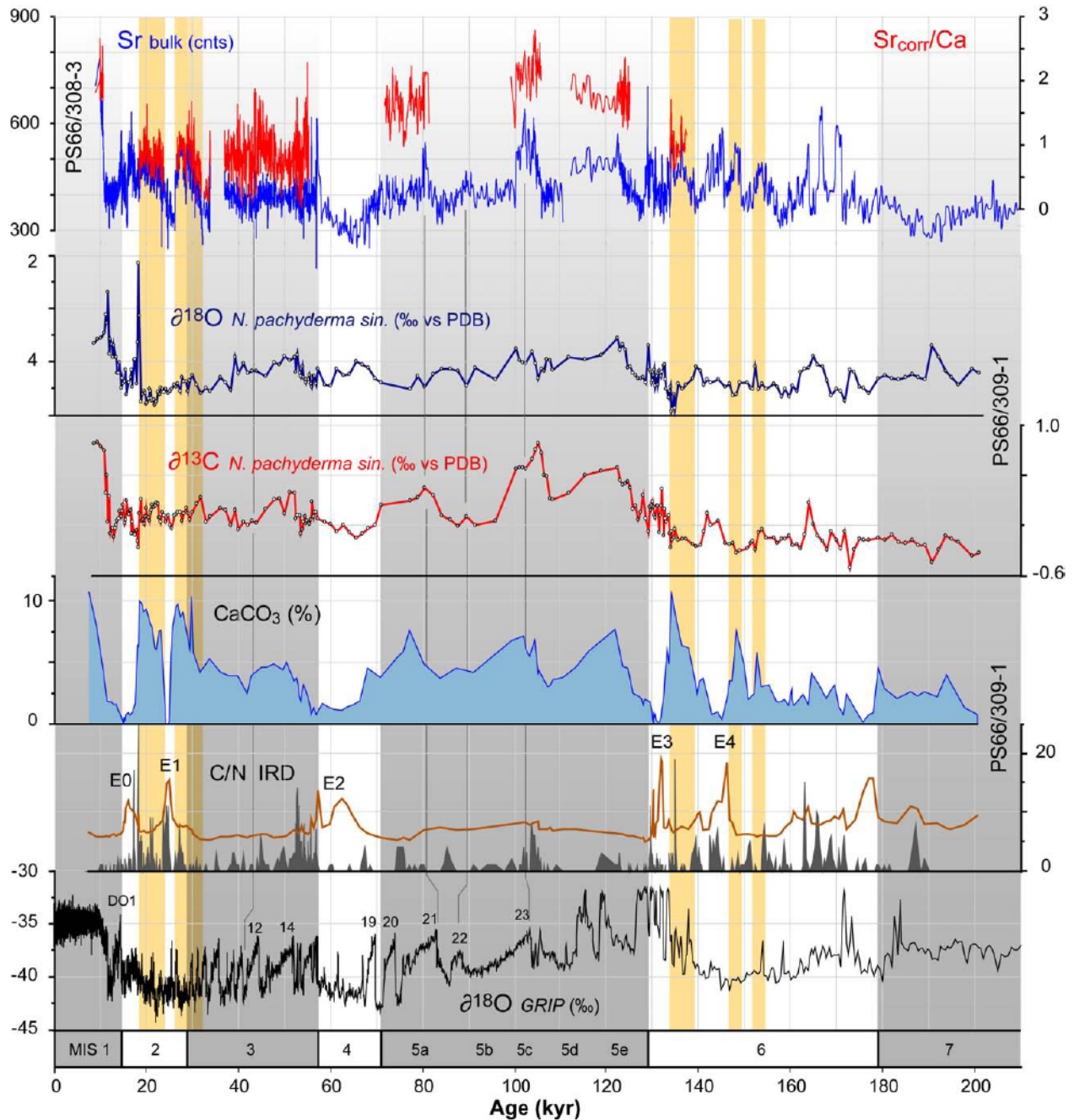
Figure 7: Core records of Sophia Basin and correlation to GRIP (Johnsen et al., 1997) showing Atlantic water inflow during high glacials (orange boxes). Note that the correlation to DO events (lines) are based on the new age model of N-GRIP (N-GRIP Ice Core Project members, 2004).
