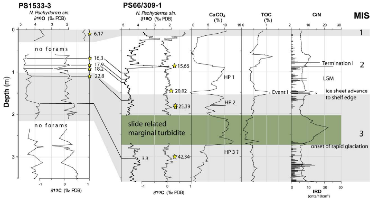
Figure 2: Proxy record of core PS66/309-1 KAL including bulk parameter and IRD for MIS 3 within Sophia Basin showing heavy stable oxygen isotope values above 4 ‰, relatively high carbonate contents during onset of Late Weichselian Glaciation and Hinlopen/Yermak Megaslides failure event. The advance to the shelf edge by the SBIS is reflected in Event I at the MIS 3/2 boundary. The interval of the Hinlopen/Yermak Megaslides failure event (marginal turbidite, green box, cf. Winkelmann et al., 2006a) follows a sudden drop to heavy \delta^{18}\text{O} values around 45 kyr. BP (MIS sub-stage 3.3). This drop might indicate the onset of the rapid glaciation. HP events (1-3) according to Hald et al. (2001). The chronostratigraphy of core PS66/309-1 KAL is based on the \delta^{18}\text{O} and \delta^{13}\text{C} record of N. pachyderma sin., the correlation to core PS1533-3 (Spielhagen et al., 2004) and AMS radiocarbon dating. Marine Isotope Stage (MIS) assignments are based on Martinson et al. (1987). AMS- 14 C dates from PS1533-3 (Nørgaard-Pedersen et al., 2003; Spielhagen et al., 2004) are correlated to PS66/309-1 KAL (left; corrected 14 C-kyr.). New AMS- 14 C dates (right; given in uncorrected 14 C-years BP) were measured on N. pachyderma sin. at the Leibniz Laboratory, Kiel University.
