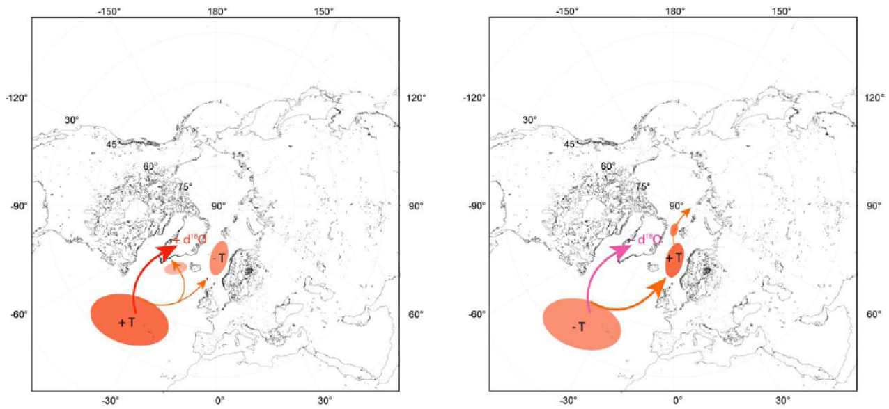
Figure 8: map with conceptual circulation models and associated thermal anomalies during step 1 and 2a: Step 1 – reduced circulation results in lighter \delta^{18}\text{O} on Greenland's ice, positive thermal anomalies in the sub-tropical N-Atlantic, SW and central Europe, negative thermal anomalies in the GIN Seas and Arctic Ocean. Step 2a – enhanced circulation cools the N-Atlantic (dynamic) heat reservoir and leads to heavier \delta^{18}\text{O} on Greenland's ice, positive thermal anomalies on NW and central Europe, within the Gin Seas and Arctic Ocean.
