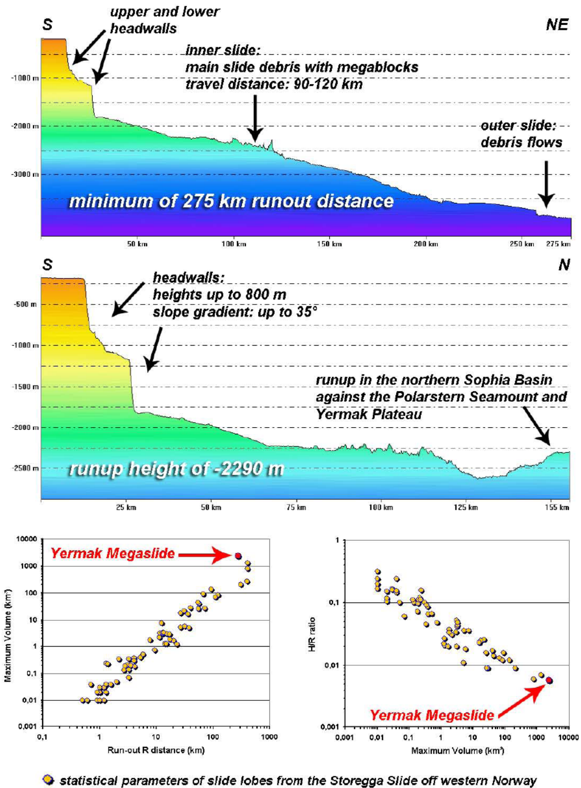
Figure 7: Bathymetric profiles (see Figure 1 for location) and geometrical parameters of the Yermak Megaslides: headwall height, runout distance, transport distance of mega blocks, slope gradients of headwalls, compared to parameters from the Storegga Slide (Haflidason et al. 2004).
