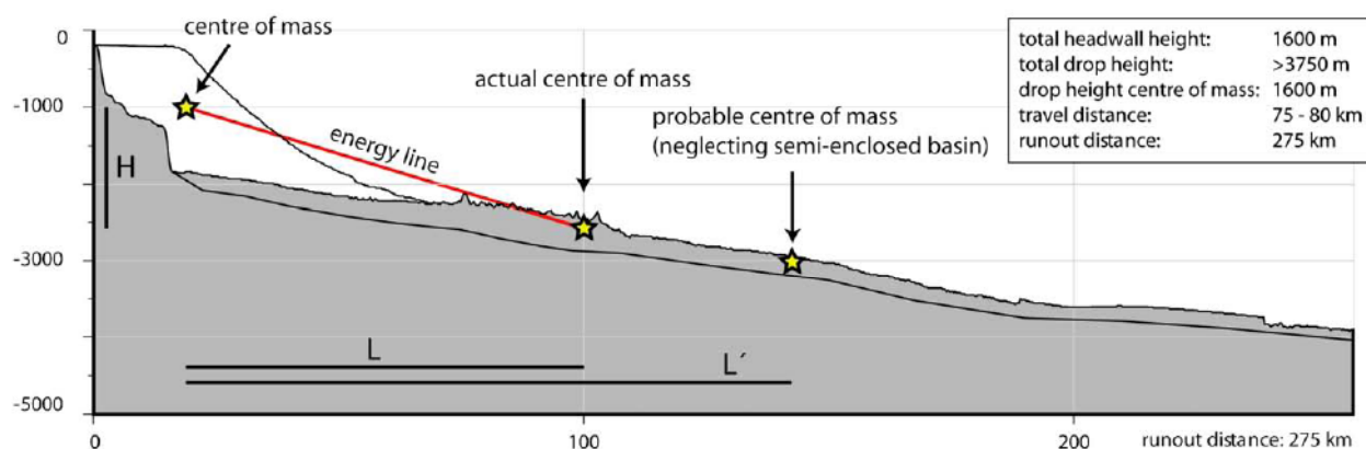
Figure 12: Energy line concept, incorporating the centre of mass of a landslide, applied to the runout profile of the Yermak Slide. Drop height (H) and travel distance (L) are based on the actual most likely centre of mass of the slided debris (area of megablocks) and the assumed shelf geometry. The travel distance for the centre of mass ( L' ) indicates a possible position of this centre if the slide would have developed into a non enclosed area. Thus L' is not constrained but remains to be modelled. Note, that the centre of mass from the evacuation area lies further to the shelf since the lateral extent is higher towards the shelf (based on Straub, 1997; modified).
