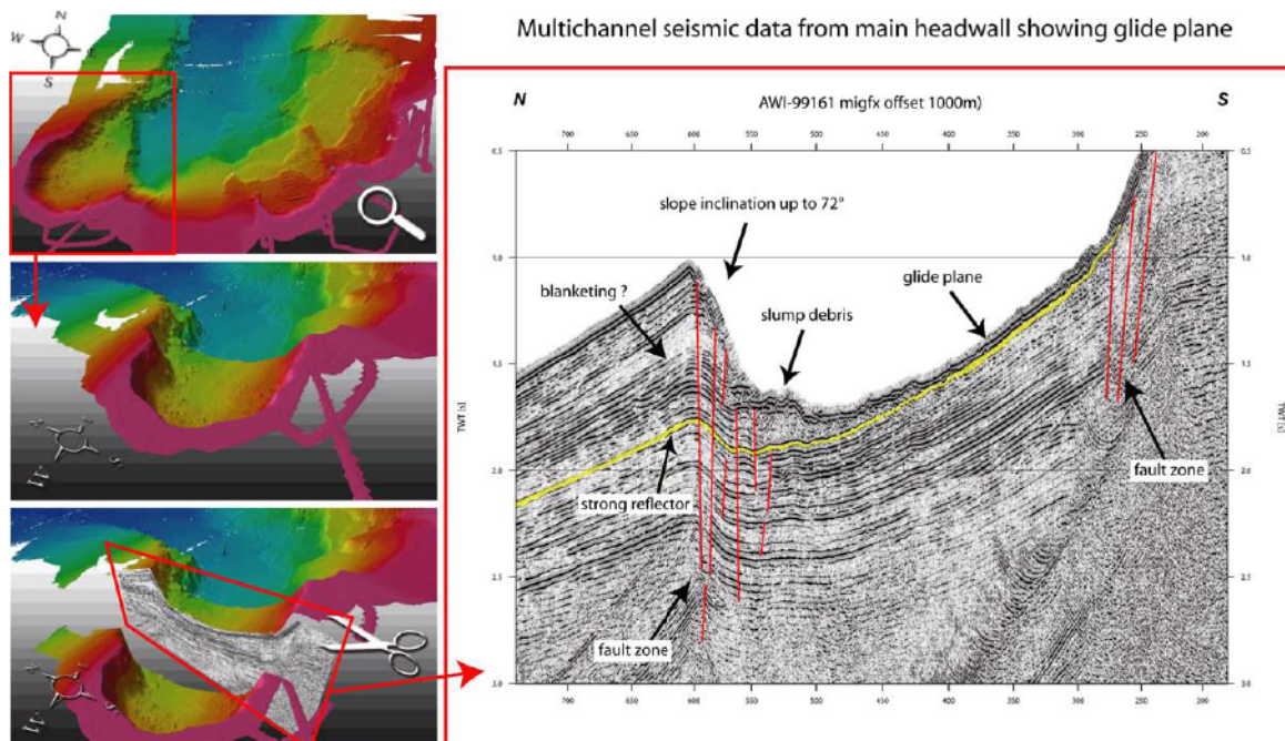
Figure 6: Seismic line AWI-99161 across the main headwall of the Hinlopen/Yermak Megalide showing slide debris on glide plane which can be traced into the adjacent fan sediments of the old Hinlopen Trough Mouth Fan. There it constitutes a strong reflector. Note that the evacuated sediment slab is bound by fault zones. The indicated blanketing results at least partly from AGC-filtering. See 3D model (view towards NE) on the left for location (seismic data from Geissler & Jokat, 2004; bathymetry data from Vanneste et al., 2006).
