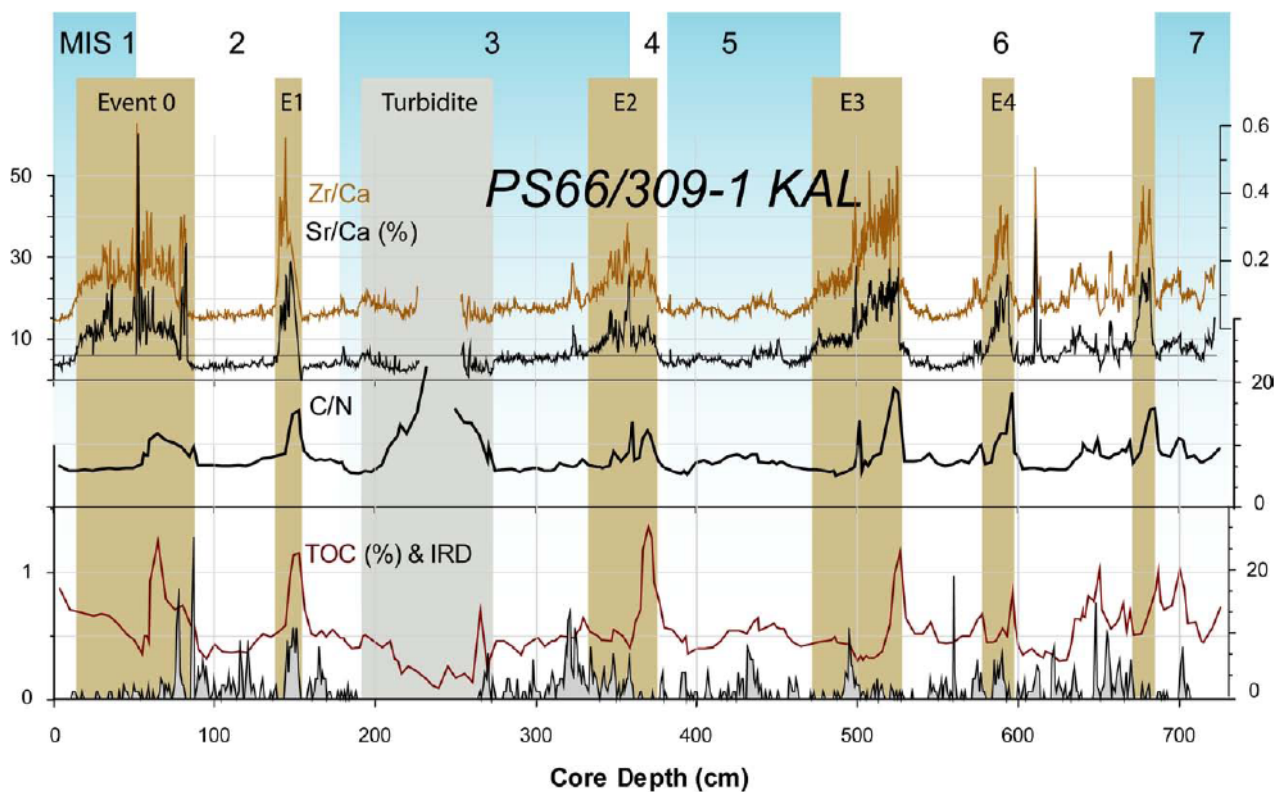
Figure 5: Terrigenous events (brown boxes) within the Sophia Basin in key core PS66/309-1. Core record of geochemical bulk parameters (TOC, C/N, CaCO 3 , Sr/Ca, Zr/Ca (XRF ratios) and IRD including indication of slide related lithological units (marginal turbidite; grey box). The peaks of the Sr/Ca ratio indicate increased input of detrital terrigenous minerals (probably plagioclase; or zircon as indicated by the Zr/Ca record, see text for explanation), from outcropping lithological strata on Svalbard (see text). Thus, the Sr/Ca ratio, here, can be used as proxy for glacial activity. Event 0 reflects Termination I; Event 1 (E1) the Late Weichselian glacial advance to the shelf edge; Event 2 (E2) the onset and termination of the Mid Weichselian Glaciation; Event 3 (E3) Termination II; and Event 4 (E4) reflects the Late Saalian glacial advance to the shelf edge during MIS 6.2. Further events within MIS 6 (e.g. Event 5, etc.) have not been named since they are less consistently recorded in our sediment cores. Note the signal offsets between C/N and Sr/Ca ratios indicating different timing of the sources (Bear Island Trough and Storfjord Trough for C/N and NE-Svalbard for the Sr/Ca ratios).
