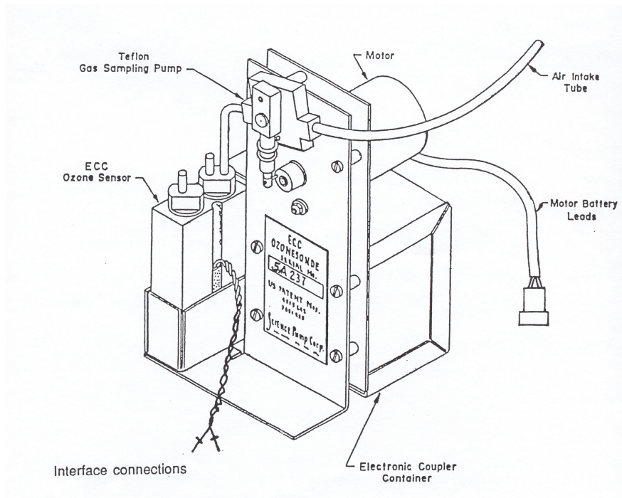
Figure 3.2: Schematic diagramme of an electrochemical concentration cell (ECC) ozonesonde, showing the principal components of the instrument
