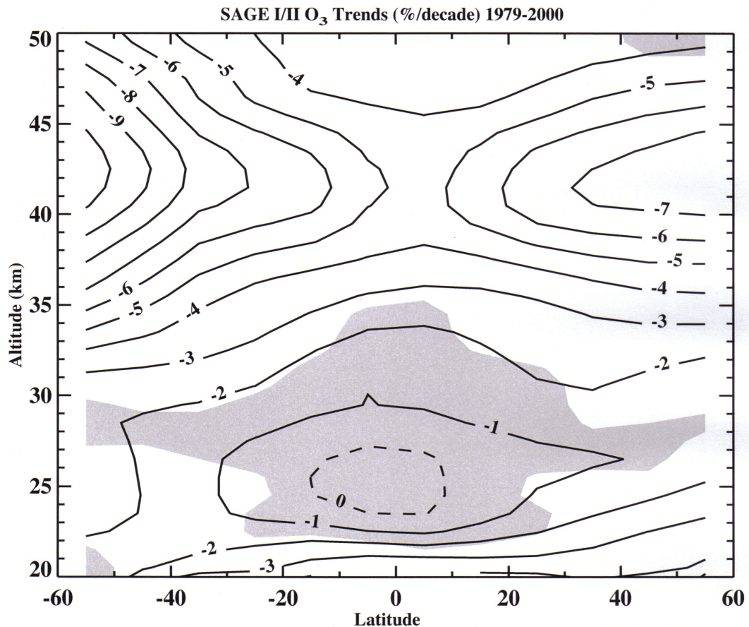
Figure 2.6: Meridional cross section of the ozone trends in percent for altitudes between 20 and 50 km. The trends are derived from the combined SAGE I and SAGE II data from 1979 to 2000, from WMO (2002).
