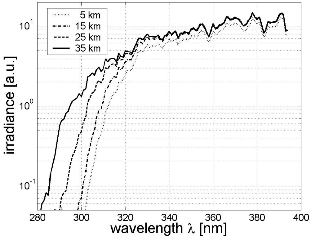
Figure 8.1: Measured spectra in the UV wavelength range from 280 to 400 nm at different altitudes between 5 and 35 km. The spectra were measured during the flight of PIOS IV, 24.6.2004 in Ny-Ålesund. The data are averaged vertically with an averaging length of 2 km and plotted every 10th kilometer.
