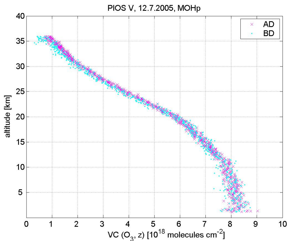
Figure 7.8: The vertical column density of ozone, calculated with the adopted Dobson algorithm for the wavelength combinations AD(magenta) and BD(cyan). Data from PIOS V flight (12.7.2005, MOHp).
