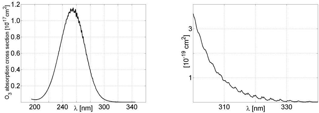
Figure 7.3: Absorption cross sections for ozone after MALICET (1995) for the wavelength range between 180 and 340 nm (left). The right panel shows an enlargement of the wavelength range between 300 and 340 nm.
