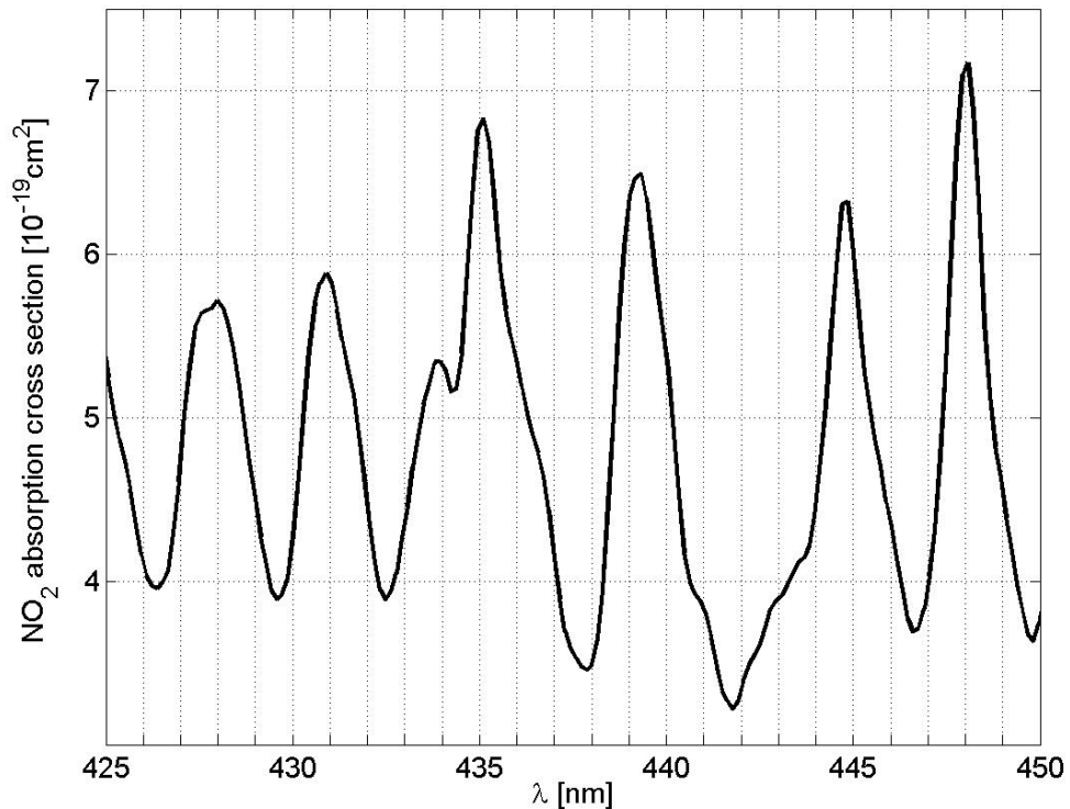
Figure 8.16: \text{NO}_2 absorption cross section in the wavelength range between 425 and 450 nm at a temperature of 223 K.
