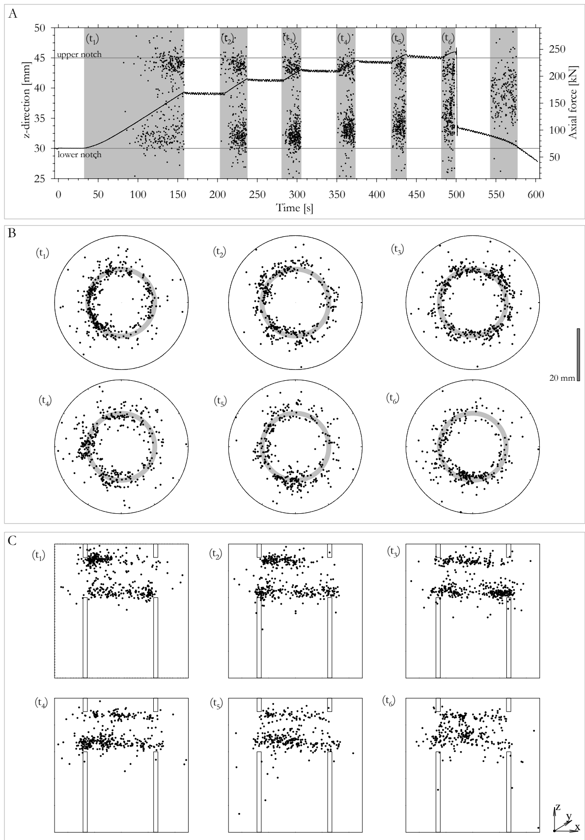
Fig. 5-27. Acoustic Emission (AE) events in space and time for Mizunami granite sample [T1-1d] at P = 30 MPa. (A) AE events successively propagate from bottom notch into sample. White areas indicate dead-time of AE acquisition system. (B) AE distribution in map view of sample for time slices from (A). Events are localised in the narrow zone between the notches. (C) Side view of sample, all events projected onto xz-plane.
