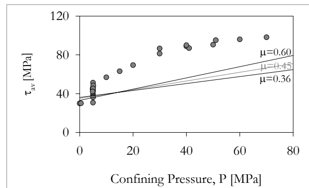
Fig. 5-32. Average shear stress at failure, \tau_{av} , vs. confining pressure, P , for Carrara marble and linear Mohr envelope for different friction coefficients. The cohesion was estimated from the UCS (uniaxial compressive strength) using the corresponding coefficient of friction; c(\mu=0.36) = 36 MPa, c(0.45) = 35 MPa and c(0.60) = 33 MPa.
