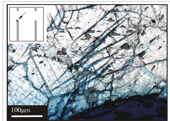
Fig. 5-20. Micrograph of the bottom notch at ~ 99 % of the maximum axial stress in Carrara marble. Only en échelon cracks are visible.
