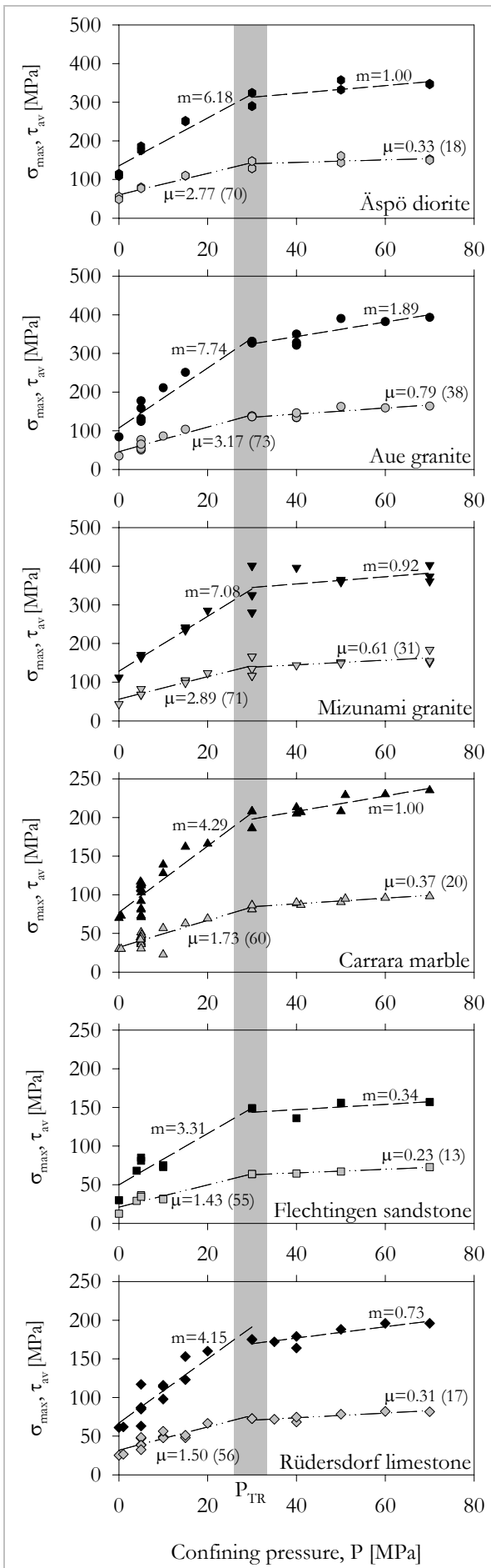
← Fig. 5-15. Influence of confining pressure, P, on \sigma_{max} and \tau_{av} for the six different rock types. The rock types are organised from top to bottom by decreasing grain size. Two regimes of different slopes are separated. m and \mu indicate slopes of regression; in brackets \Phi = \arctan \mu is given. Black symbols: \sigma_{max} , grey symbols: \tau_{av} . Grey vertical mark indicates transitional regime. [W=50mm, D=50mm, a=5mm, IP=15 mm].
