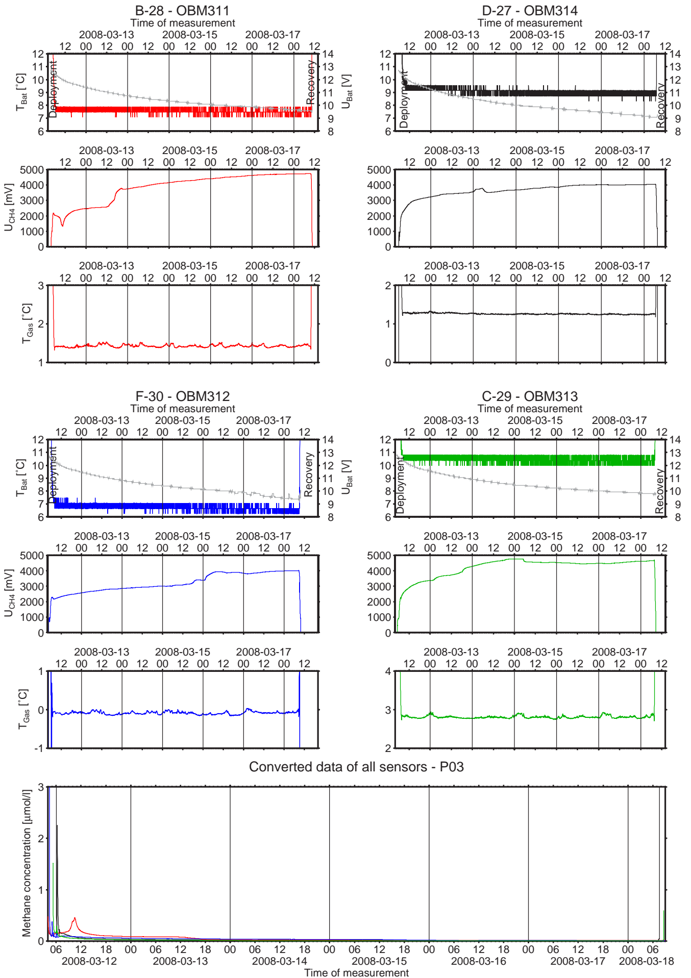
Fig. 12.4: Upper four diagrams-sections display temperature ( T_{Bat} in color) and voltage ( U_{Bat} in grey) of the batteries, methane voltage ( U_{CH4} ), and gas temperature ( T_{Gas} ), respectively for each sensor. Lower diagram shows the methane concentration for all four sensors.
