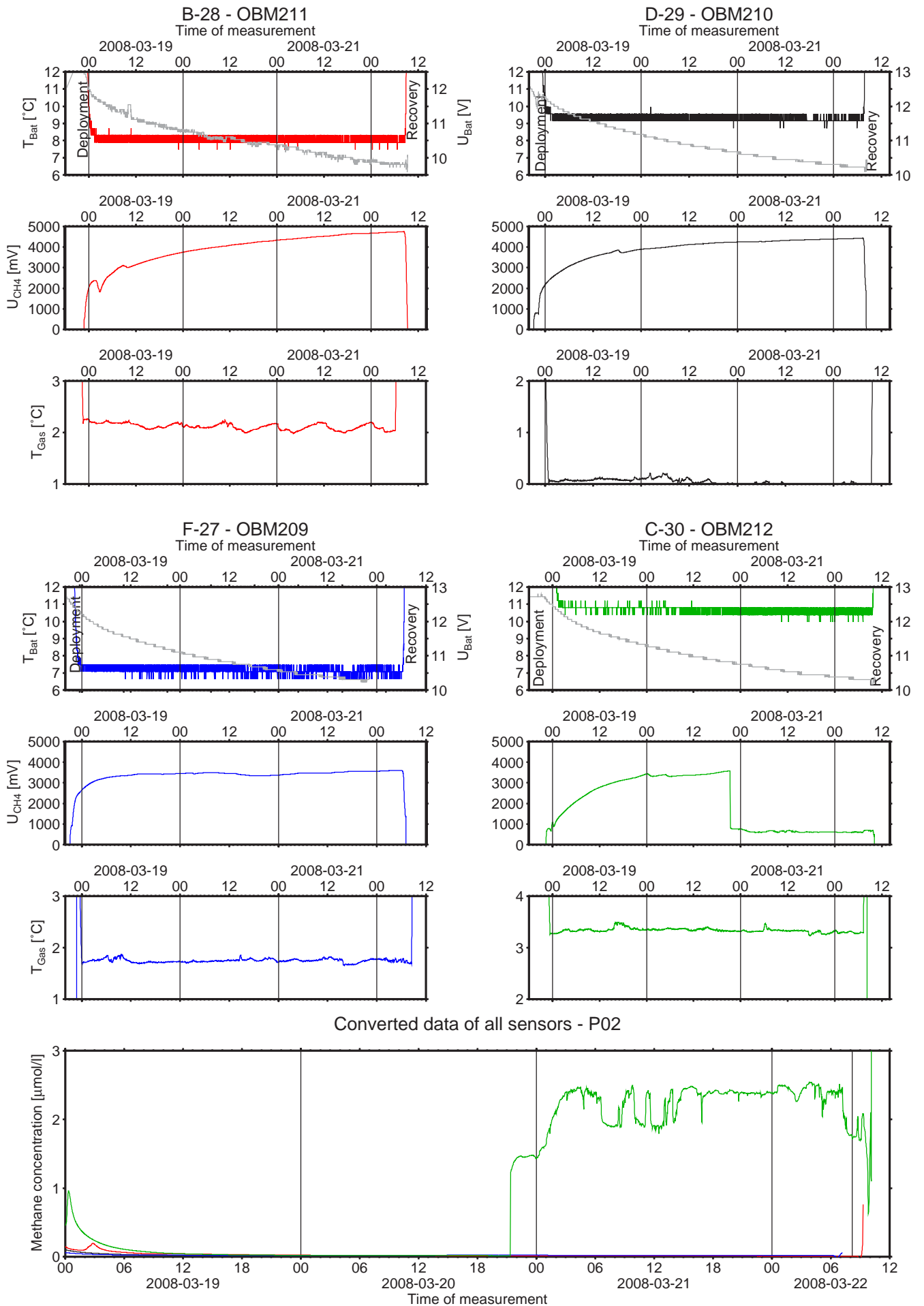
Fig. 12.3: Upper four diagrams-sections display temperature ( T_{Bat} in color) and voltage ( U_{Bat} in grey) of the batteries, methane voltage ( U_{CH4} ), and gas temperature ( T_{Gas} ), respectively for each sensor. Lower diagram shows the methane concentration for all four sensors.
