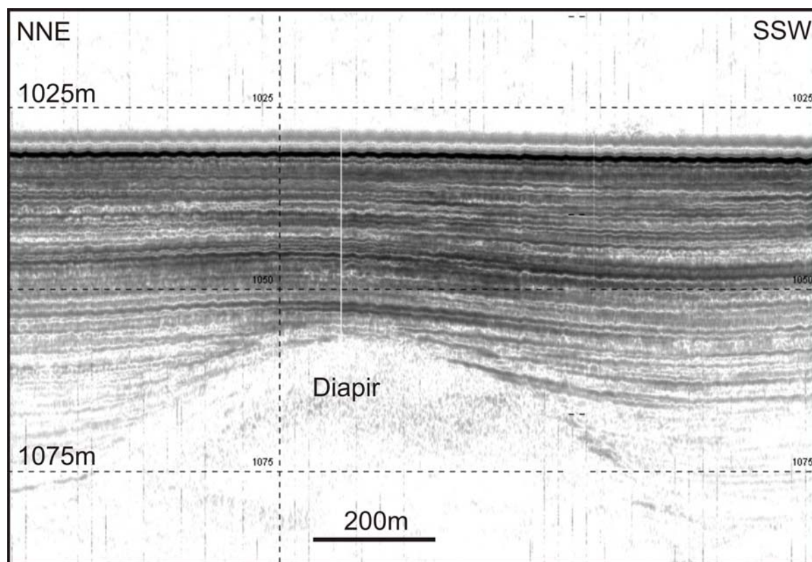
Fig. 5.4.5: Sub bottom profiler data showing a diapiric structure beneath well stratified sediments. See Fig.5.4.1 for location.
