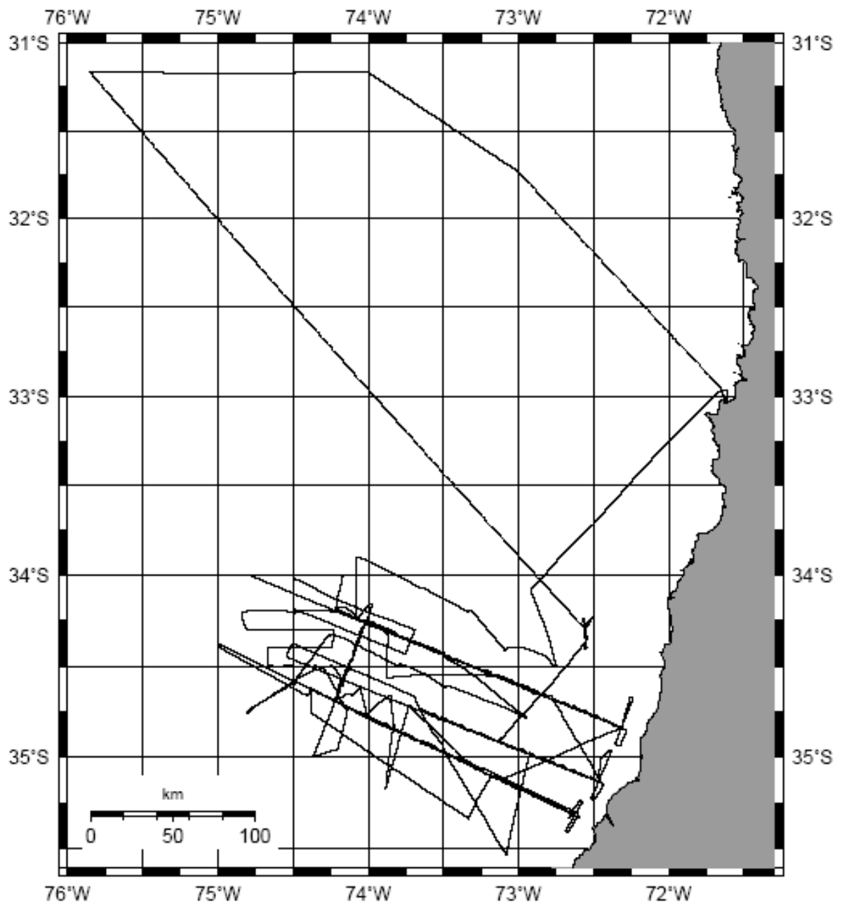
Figure 4.1.: Track chart of cruise JC23 Leg 1
