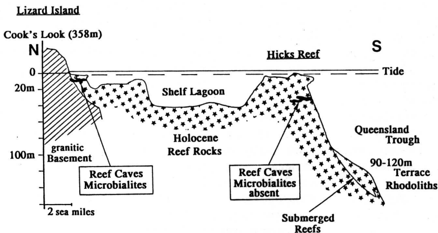
Fig. 10. Simplified N-S profile Lizard Island Hicks-Reef
