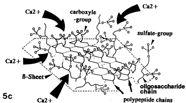
Fig. 5. Mineralization model via Ca-binding organic macromolecules.
