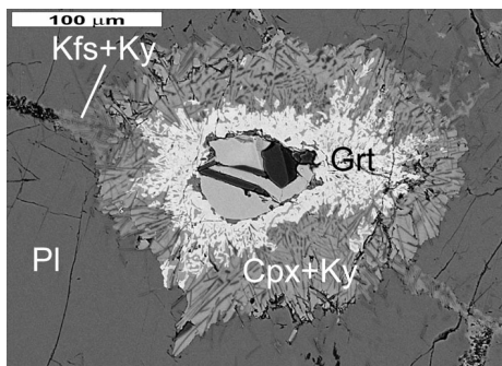
Figure 1: Eclogite facies garnet-omphacite-kyanite corona around spinel/corundum embedded in a plagioclase groundmass within an otherwise unreacted granulite facies anorthosite. The grain boundaries between plagioclase grains show tiny growth of K-feldspar and kyanite.
