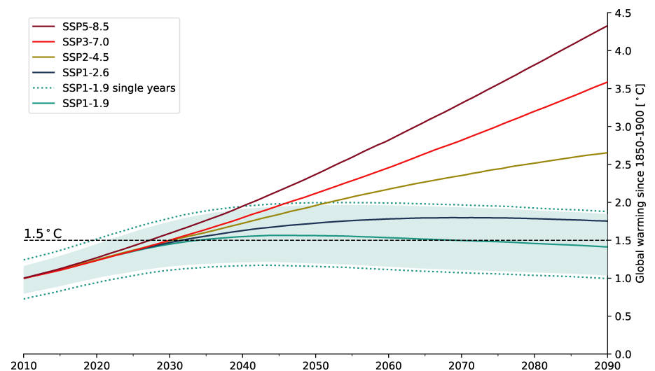
Figure 1. Future global warming depends on how emissions evolve and thus on humans' decisions. Each colour corresponds to one particular scenario of future emissions, ranging from very low CO 2 emissions (implying rapid, strong, and sustained emissions reductions; green) to very high CO 2 emissions (dark red). Shown are global warming levels as a function of time, for each scenario; note that since global warming is defined as an average over twenty years, the years on the x-axis indicate the midpoint of a twenty-year period. The curves show the most likely temperature for a given time and a given scenario; the green shading indicates the uncertainty range for the very low scenario, arising from uncertainty in climate sensitivity and historical warming. For the other scenarios, the uncertainty ranges are roughly similar but somewhat larger. The dotted line represents the additional uncertainty if year-to-year fluctuations are considered. Single-year exceedance of 1.5 degC could occur before the 1.5 degC global warming level would be reached.
