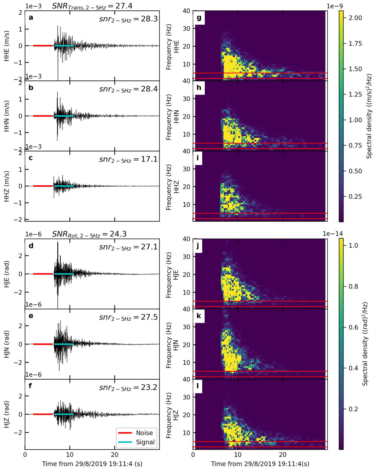
Figure 3. (a–f) Seismograms and (g–l) spectrograms of a MI 1.9 volcano-tectonic event close to the main craters at 19:11 on 29 August. Panels (a–c and g–i) show the seismometer data and (d–f and j–l) the rotational sensor data for the E , N , and Z component. Note the different amplitude and color scale to aid visual comparison of the events recorded by different sensor types, especially for the spectral density. In panels (a–f) the horizontal lines mark a 4 s window duration for the noise (red) and signal (cyan) in the signal-to-noise ratio (SNR) ratio calculation. The mean SNR (Equation 2) can be found on top of the seismograms while we display the SNR for each component (Equation 1) in the right upper corner of each seismogram. In panels (g–l) the red lines mark the frequency band of the SNR calculation.
