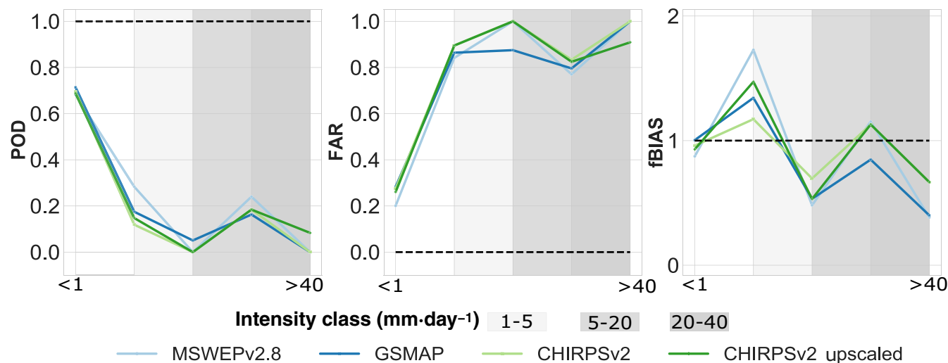
FIGURE 7 Median values of probability of detection (POD), false alarm ratio (FAR), and frequency of bias (fBias) performance for dry spells (<1 mm-day -1 ) and wet spells of different intensities (1–5, 5–20, 20–40, and >40 mm-day -1 ). The horizontal dashed line indicates the optimum POD, FAR, and fBIAS values [Colour figure can be viewed at wileyonlinelibrary.com ]
