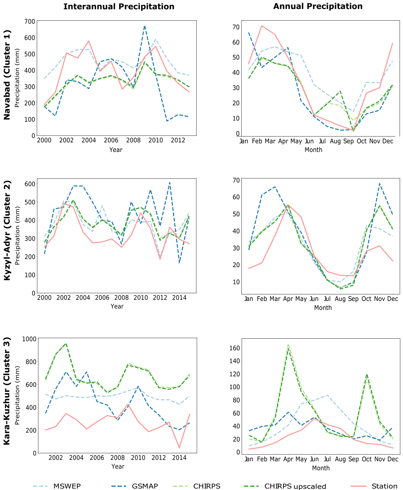
FIGURE 6 Interannual variation in precipitation and annual precipitation estimated by the precipitation products (dashed lines), as compared to the gauging stations (solid lines) for each cluster. Cluster 1 (winter/spring precipitation; long, dry summers); cluster 2 (winter/spring precipitation; short, dry summers), and cluster 3 (summer precipitation) [Colour figure can be viewed at wileyonlinelibrary.com ]
