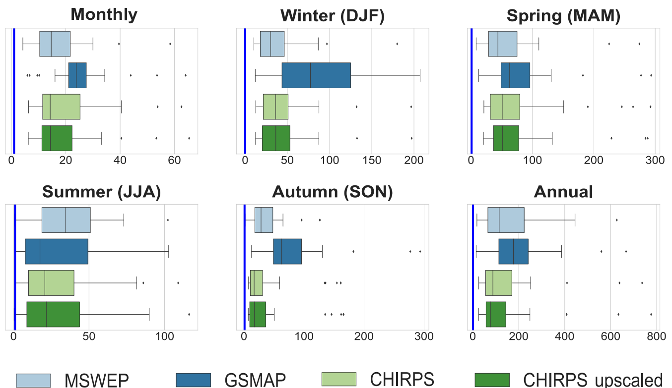
FIGURE 3 Mean absolute error (MAE) in mm of various global precipitation datasets and precipitation gauge data for six different temporal scales. The vertical blue line indicates the optimum value for MAE [Colour figure can be viewed at wileyonlinelibrary.com ]
