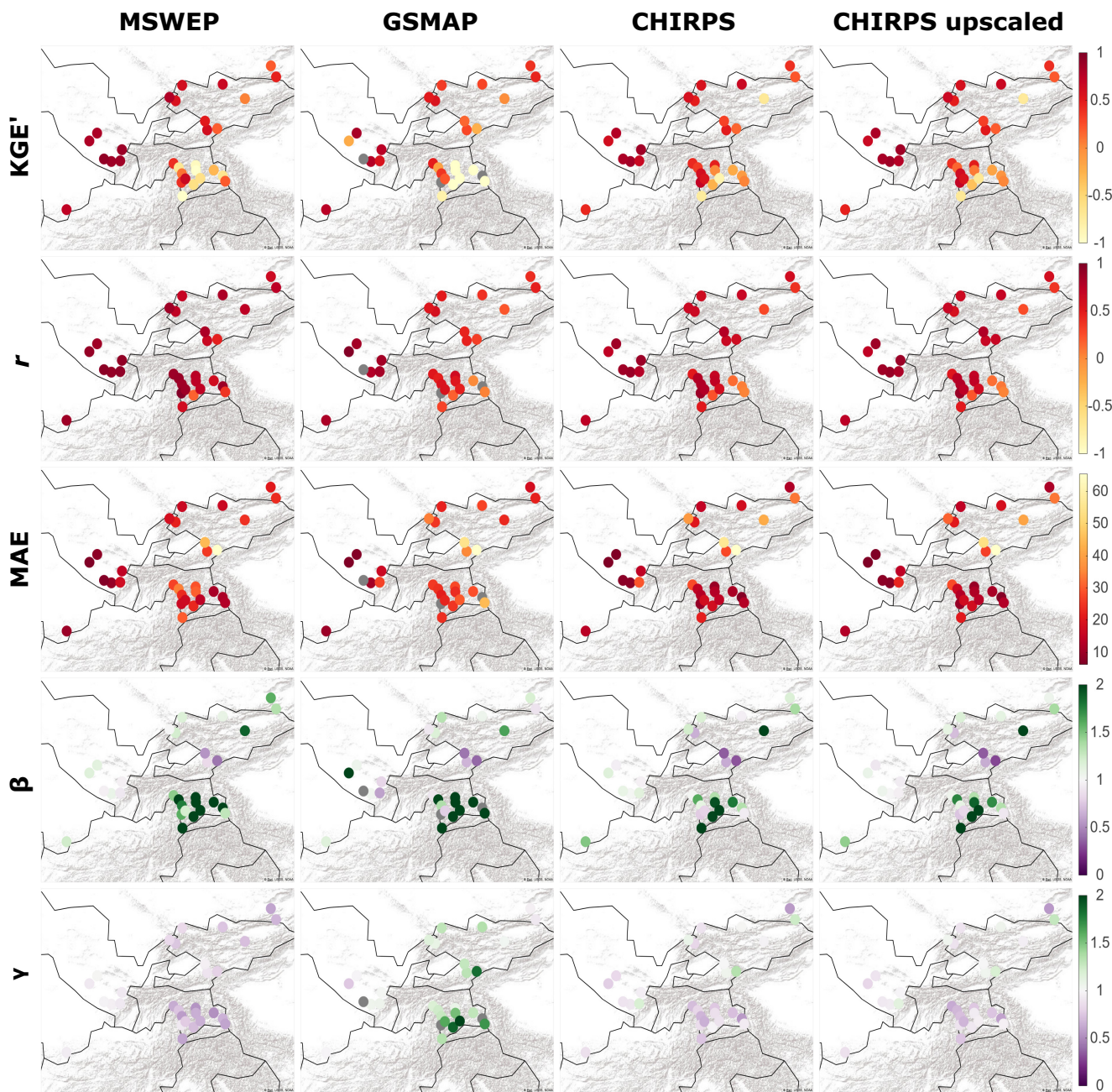
FIGURE 4 KGE', its components ( r , \beta , \gamma ), and MAE derived from a monthly timescale. The colours for KGE', r , and MAE range from light yellow (very poor performance) to dark red (best performance). For \beta and \gamma , white colours represent their best performance, while underestimation is depicted in dark purple and overestimation is depicted in dark green. Grey colour identifies stations not available for product evaluation (i.e., GSMAP, data before 2000). The black outlines correspond to the countries (see Figure 1 for a detailed map of the region) [Colour figure can be viewed at wileyonlinelibrary.com ]
