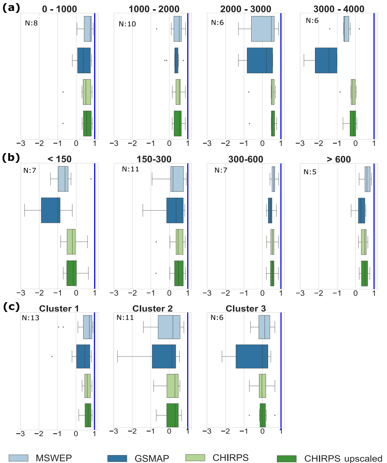
FIGURE 5 KGE' at a monthly timescale between the precipitation products and precipitation gauge data for different (a) elevation bands: 0–1,000 m, 1,000–2,000 m, 2,000–3,000 m, and 3,000–4,000 m; (b) mean annual precipitation (2000–2015); (c) precipitation regimes with corresponding clusters (cluster 1 has winter–spring precipitation, long dry summers; cluster 2 has winter–spring precipitation, short dry summers, and cluster 3 is characterized by summer precipitation). The vertical blue line indicates the optimum value for KGE' . N indicates the number of stations in each group [Colour figure can be viewed at wileyonlinelibrary.com ]
