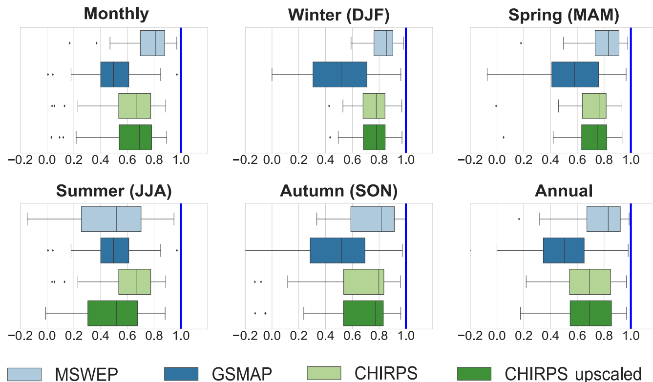
FIGURE 2 KGE' between the precipitation products and precipitation gauge data for six different timescales. The vertical blue line indicates the optimum value for KGE' . From left to right and up to bottom: monthly, winter (December, January, February), spring (March, April, May), summer (June, July, August), and autumn (September, October, November) [Colour figure can be viewed at wileyonlinelibrary.com ]
