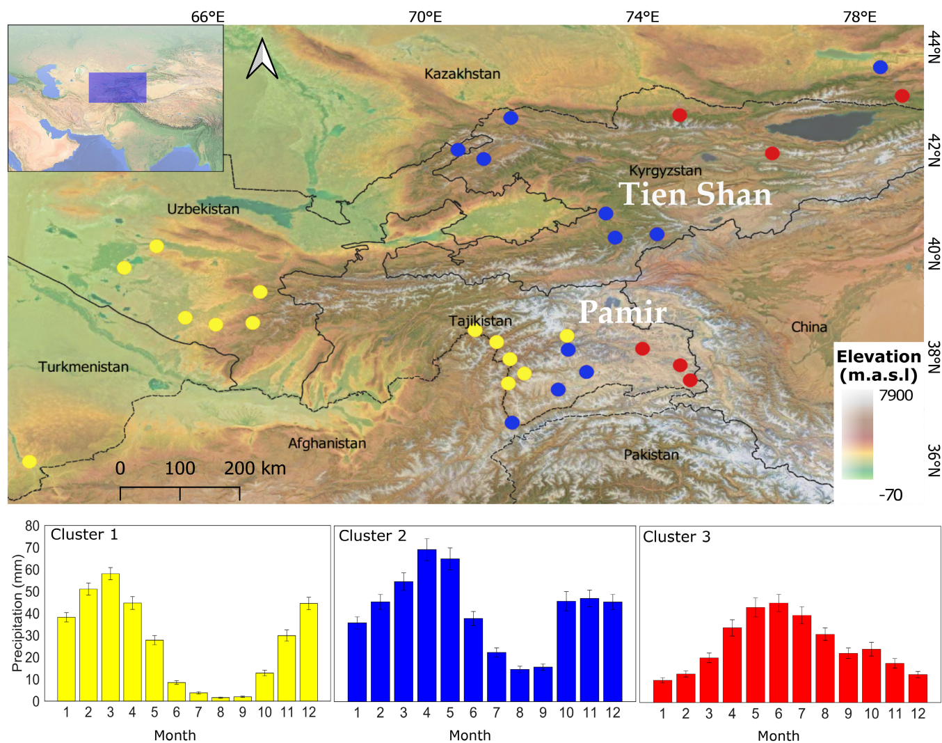
FIGURE 1 Study area and location of the 30 precipitation stations used for validation. Bar plots represent the annual precipitation regimes (section 4.4) of the clusters shown in the map: cluster 1 (yellow) is characterized by winter and spring precipitation and long, dry summers and autumns; cluster 2 (blue) has winter and spring precipitation and a short, dry summer period; and summer precipitation dominates in cluster 3 (red) [Colour figure can be viewed at wileyonlinelibrary.com ]
