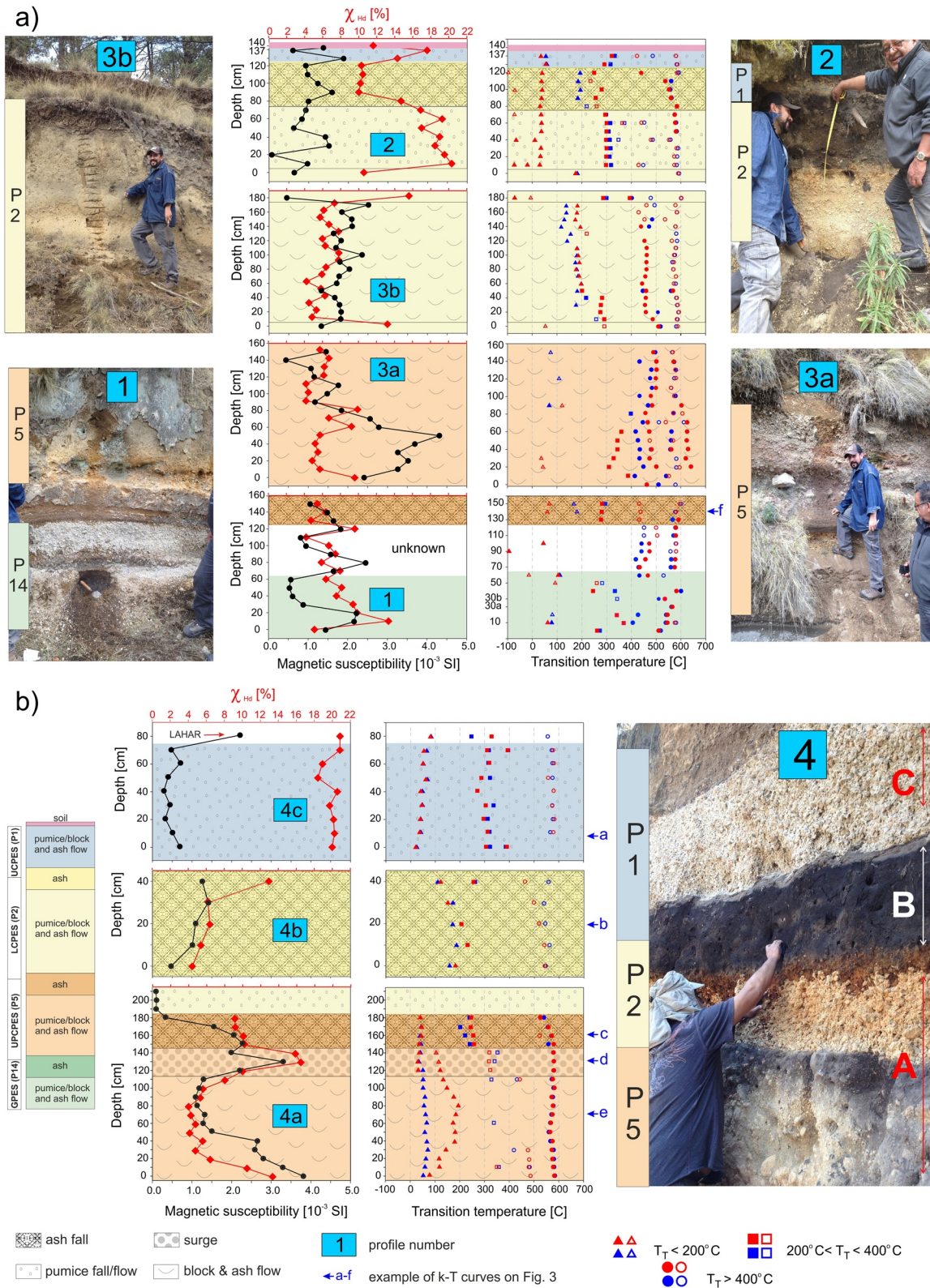
Figure 2. Changes in magnetic susceptibility (black) and field dependence (red) parameter (left column) and transition temperatures (right column) with depth for the different profiles along the Paso de Cortés road. Stratigraphic positions are shown in the field photographs and data profiles. Filled symbols in the right columns represent the transition temperatures of the dominant phase, whereas open symbols describe the minor phases derived from \kappa(T) curves. Red and blue indicate temperatures obtained from heating and cooling curves, respectively. The field dependence parameter ( \chi_{Hd} ) was calculated according to Equation 1. Small blue arrows with letters (on the right) indicate the location of \kappa(T) curves shown in Figure 3. For an explanation of abbreviations, see Figure 1.
