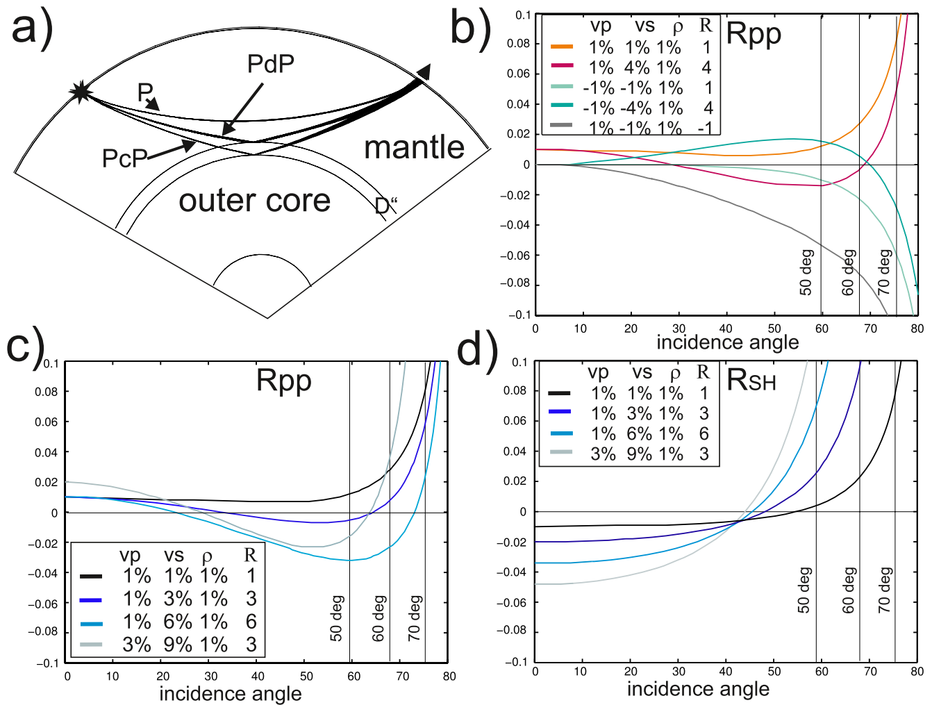
Figure 1. (a) Wave paths of P waves, the reflection off the D'' discontinuity PdP , and PcP , the CMB-reflected phase. Same paths for S , SdS , and ScS . (b) Reflection coefficient for P to P reflections ( R_{pp} ) at the D'' discontinuity with variable changes in V_p , V_s and density across the reflector as given in the legend. (c) Same as for (b) but for different (but only positive) values of the changes in V_p and V_s across D'' . (d) Same as (c) but for SH to SH reflection coefficient ( R_{SH} ). The distance corresponding to the incidence angle at the discontinuity is given by the vertical lines in (b–d).
