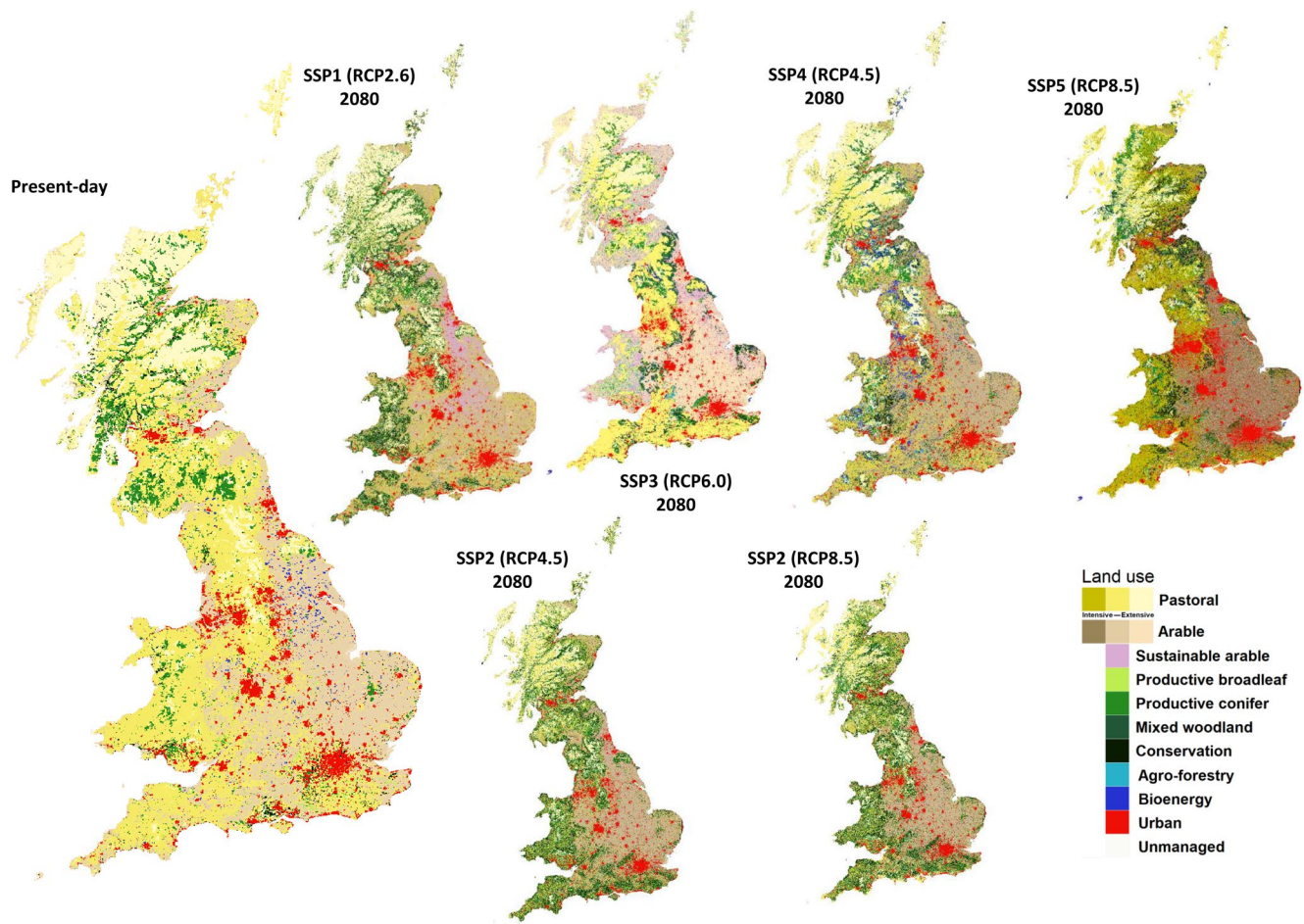
Figure 3. Maps of amalgamated agent types in 2080 in each RCP-SSP combination.
