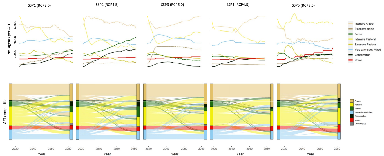
Figure 5. Agent Functional Type (AFT) dynamics throughout each SSP scenario: numbers of agents within amalgamated AFTs (top) and transitions between broad land use types (bottom). RCP8.5-SSP2 results were very similar to those shown for RCP4.5-SSP2, and can be found in Figure S11 in Supporting Information S1.
