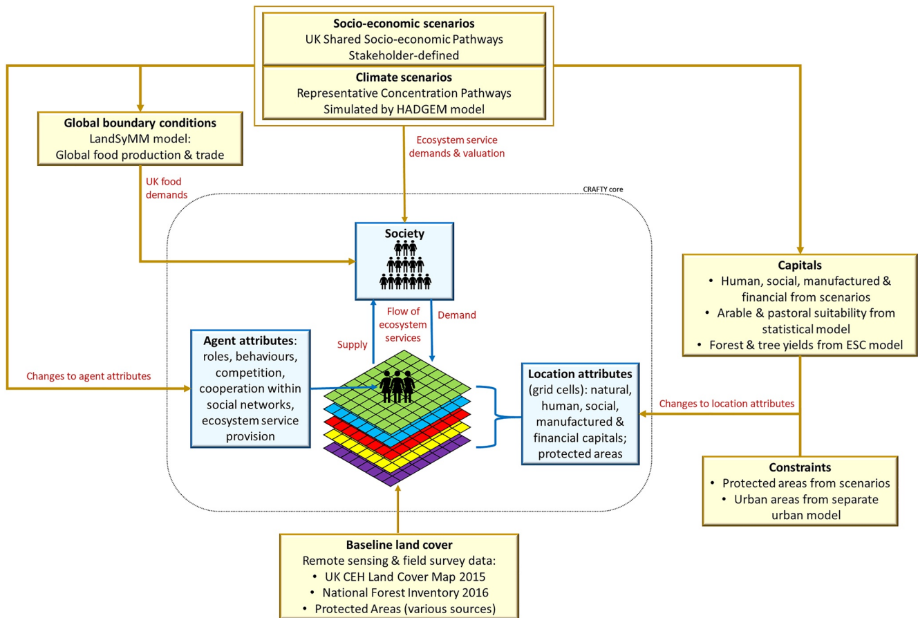
Figure 1. Schematic diagram of CRAFTY-GB structure and information flows. The blue features belong to the generic core of CRAFTY, and the yellow features are specific to the British model implementation, providing information to the core processes. This external information is derived from observational, modeled and stakeholder-developed data explained in detail in Supporting Information S1. Red labels describe particular information exchanges.
