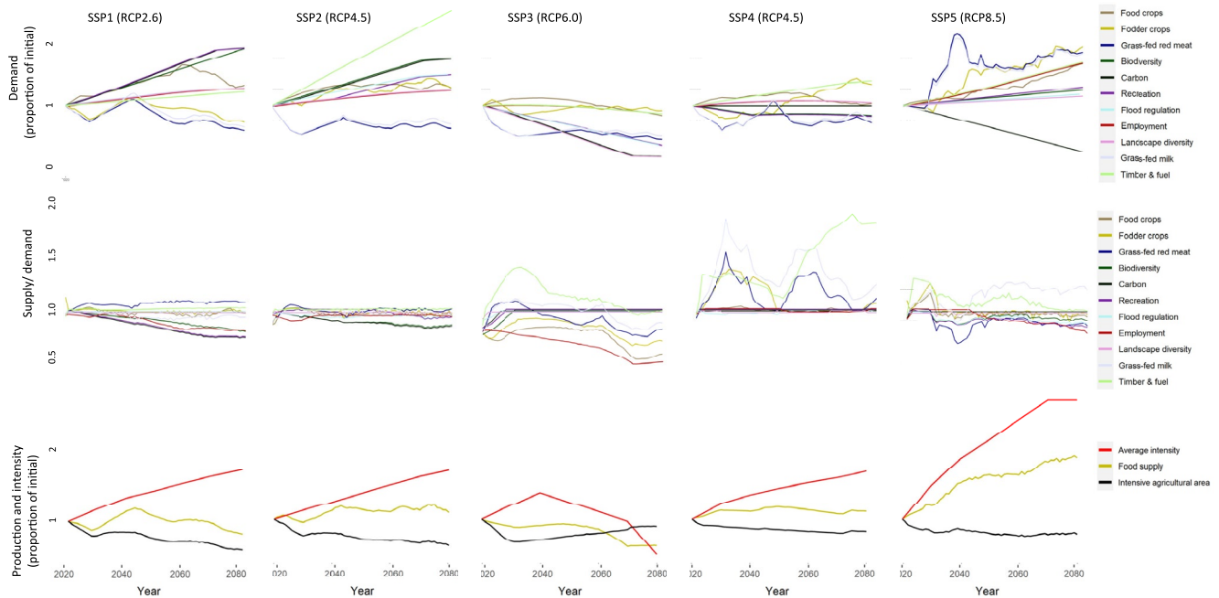
Figure 4. Demand levels, supply as proportion of demand, and land use intensity, food supply and intensive area throughout each SSP scenario (RCP8.5-SSP2 results were very similar to those shown for RCP4.5-SSP2, and can be found in Figure S11 in Supporting Information S1).
