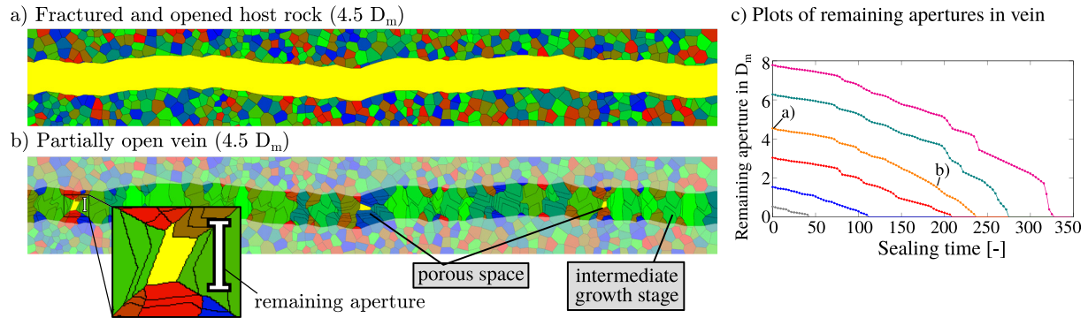
Figure 3. Single-seal veins in larger setup: (a) Opened fracture. (b) Partially sealed vein. Inset shows remaining aperture, which is used for probabilistic simulations. Black lines indicate intermediate growth stages, host rock is highlighted in light gray. (c) Plots of remaining aperture in veins with different apertures.
