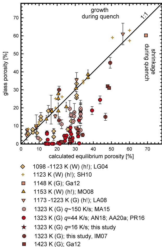
Fig. 11 Observed glass porosities vs. calculated equilibrium porosities for all decompression experiments with hydrous phonolitic melt composition, in which near-equilibrium degassing was facilitated prior to quench. (G) gas as pressure medium, (W) water as pressure medium. When q and error bars are not given, they are unknown. (h!) hydration vesicles might have been present prior to decompression due to the use of powder as starting material and H_2O supersaturated conditions prior to decompression. The experiments with melts containing hydration vesicles are the only ones plotting close to the 1:1 line, suggesting that no vesicle shrinkage occurred. The presence of a pre-existing fluid phase, however, can shift the glass porosities of the quenched samples to higher values towards or above the 1:1 line, although shrinkage occurred. Additionally, other reasons might also influence the glass porosity of these samples (see text). All data of other samples plot below the 1:1 line indicating vesicle shrinkage during cooling. A faster cooling rate ( 150\text{ K}\cdot\text{s}^{-1} ) leads to slightly less shrinkage (MA15) compared to slower cooling ( 44\text{--}16\text{ K}\cdot\text{s}^{-1} ; this study) References: LG04: Larsen and Gardner (2004); SH10: Shea et al. (2010); GA12: Gardner (2012); MO08: Mongrain et al. (2008); LA08: Larsen (2008); MA15: Marxer et al. (2015); AN18: Allabar and Nowak (2018); AA20a: Allabar et al. (2020); PR16: Preuss et al. (2016); IM07: Iacono-Marziano et al. (2007). Compilation of data can be found in the online resource “Literature Review”
