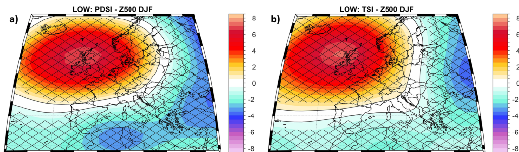
Fig. 6 Large-scale climate drivers of dry events. a The low composite map between the reconstructed 21 PDSI index (PDSI < −0.75 std. dev.) and winter reconstructed Geopotential Height at 500 mb (Z500) 53 and (b) the low composite map between the reconstructed TSI 63 (TSI < −0.75 std. dev.) and winter reconstructed Geopotential Height at 500 mb (Z500) 53 . The hatching highlights significant values at a confidence level of 95%. Analyzed period: 1500–1999. Units: Z500 (m).
