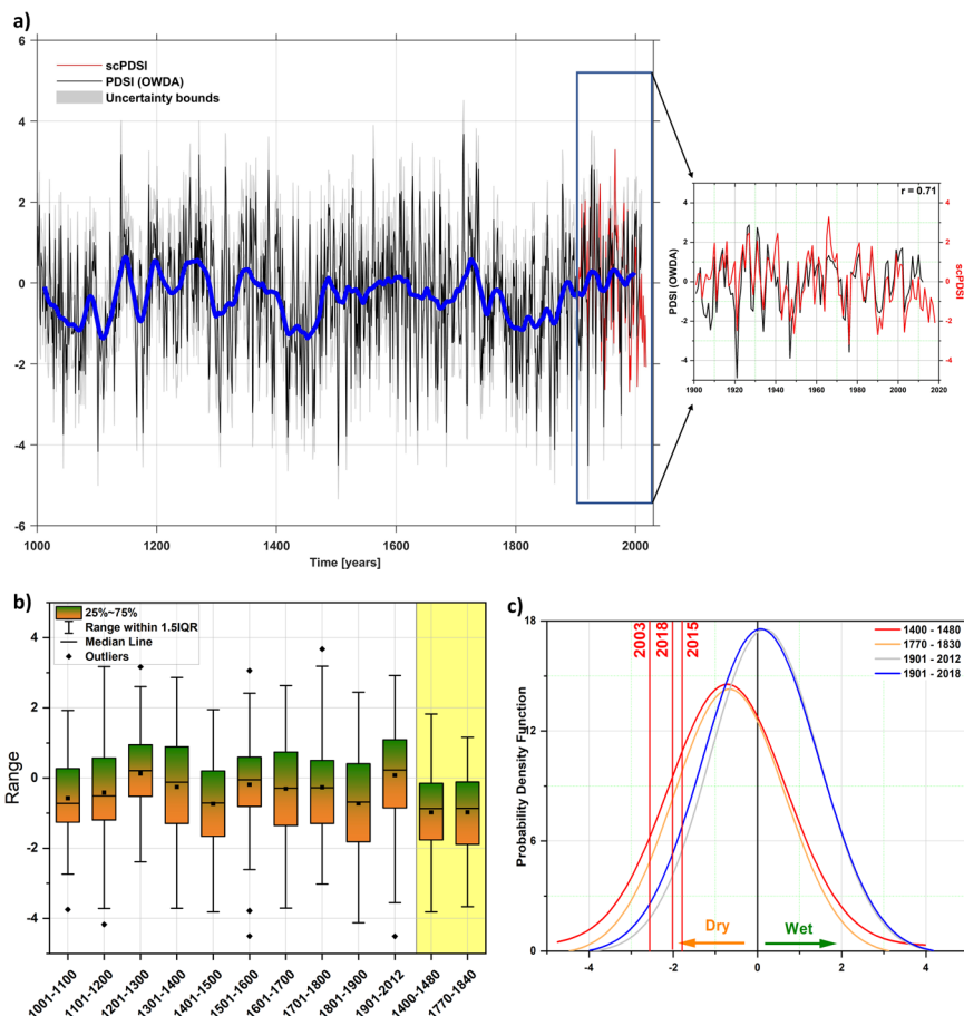
Fig. 2 Drought events from a long-term perspective. a Regional mean Old World Drought Atlas (OWDA) 21 PDSI index for central Europe (3°E–20°E, 45° N–56°N, black line) for the 1000–2012 period and the instrumental 50 June through August scPDSI (solid red line) for the 1901–2018 period. Uncertainty ( 1\sigma ) calculated as the root-mean-squared error from the residual fit to the instrumental series shown as the shaded gray region. The blue line represents the 31 years running mean of the OWDA time series; (b) Comparison between the reconstructed PDSI index (black line) 21 and the observed scPDSI index (red line) 50 over the common period: 1901–2012; (c) The fitted Gaussian distribution of the reconstructed PDSI 21 values for different time periods: 1400–1480 (red line), 1770–1840 (orange line), 1901–2012 (gray line) and for the observational data 50 for the period 1901–2018 (blue line). The values for 2003, 2015, and 2018 are indicated with a red line. The OWDA record has been adjusted by the mean and standard deviation so that it has the same mean and standard deviation as the instrumental data.
