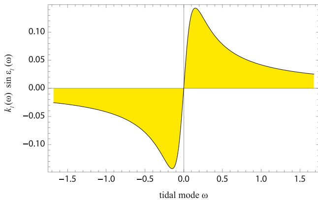
Figure 1. A typical shape of the quality function K_f(\omega) = k_f(\omega) \sin \epsilon_f(\omega) , where \omega is a shortened notation for the tidal Fourier mode \omega_{mpq} (from Noyelles et al., 2014).
