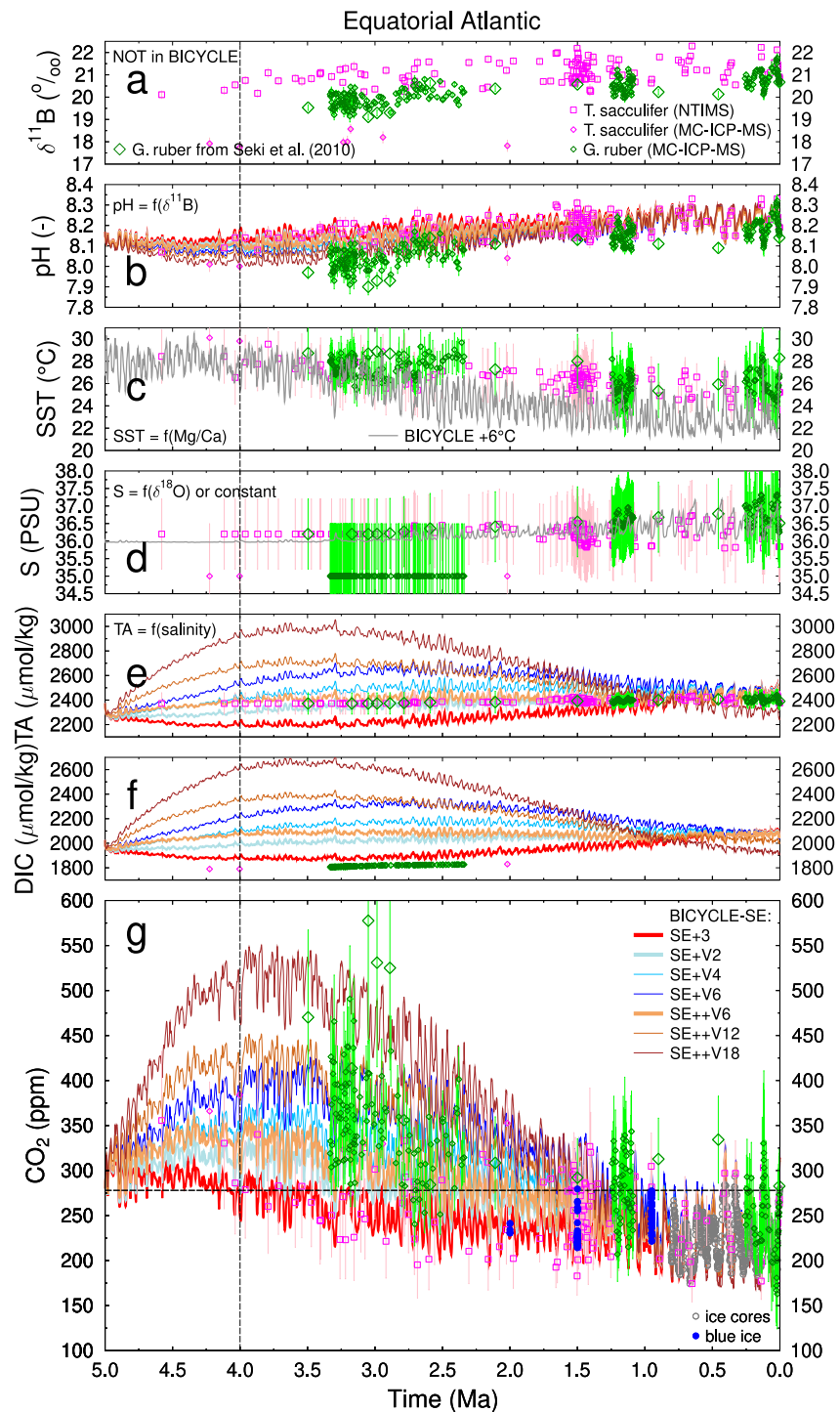
Figure 4. Details on the \delta^{11}\text{B} -based \text{CO}_2 proxies from the surface equatorial Atlantic (see legends in subfigures a and g): (a) measured \delta^{11}\text{B} ; (b) \text{pH} ; (c) sea surface temperature; (d) salinity; (e) TA; (f) DIC; (g) atmospheric \text{CO}_2 . Data as compiled in Dyez et al. (2018) with updates from de la Vega et al. (2020) and paleo-co2.org with additions of \text{CO}_2 from ice cores (Bereiter et al., 2015) and blue ice (Yan et al., 2019). As 2nd variable of the carbonate system nearly all studies estimates TA, while de la Vega et al. (2020) estimates dissolved inorganic carbon. Data originally published in Seki et al. (2010) are marked with different symbols, since they contain the unusual high \text{CO}_2 values around 3 Ma. All uncertainties are \pm 1\sigma .
