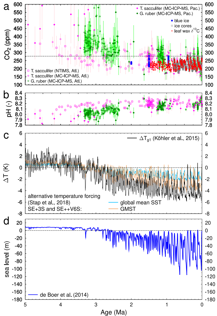
Figure 1. Climate reconstructions over the past 5 Ma. (a) Atmospheric CO 2 concentration and (b) surface water pH reconstructed from \delta^{11}\text{B} , distinguished by species, method and ocean basin (Atlantic: open symbols; Pacific: filled symbols). Based on Atlantic cores as compiled in Dyez et al. (2018) with updates from de la Vega et al. (2020) and Pacific core as in Guillermic et al. (2022); In (a) additionally data from ice cores (Bereiter et al., 2015), blue ice (Yan et al., 2019) and leaf wax \delta^{13}\text{C} (Yamamoto et al., 2022) are plotted. (c) Global temperature changes: \Delta T_{g1} is taken from (Köhler et al., 2015b) and represents a global mean surface temperature (GMST), alternative data from Stap et al. (2018a) (GMST; global mean sea surface temperature) are taken; (d) Sea level (de Boer et al., 2014). Error bars show 1\sigma uncertainties.
