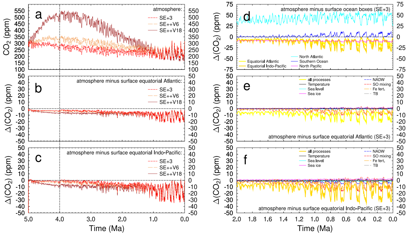
Figure 3. The difference between atmospheric CO 2 concentration and pCO 2 in surface waters. Atmospheric CO 2 concentration (a) and the difference to equatorial pCO 2 in surface waters (b: Atlantic; c: Indo-Pacific) for three selected scenarios (SE+3; SE++V6; SE++V18). (d–f): Zoom-in on the last 2 Ma for scenario SE+3 including contributions of individual processes to the differences in the equatorial boxes. (d) All surface ocean boxes; (e): equatorial Atlantic; (f): equatorial Indo-Pacific. The process of interest is switched off and the results subtracted from the control run with all processes active. The investigated processes are ocean temperature, sea level, sea ice, strength of the North Atlantic Deep Water (NADW) formation, vertical mixing in the Southern Ocean (SO), iron fertilization in the Southern Ocean, and changes in the terrestrial biosphere (TB).
