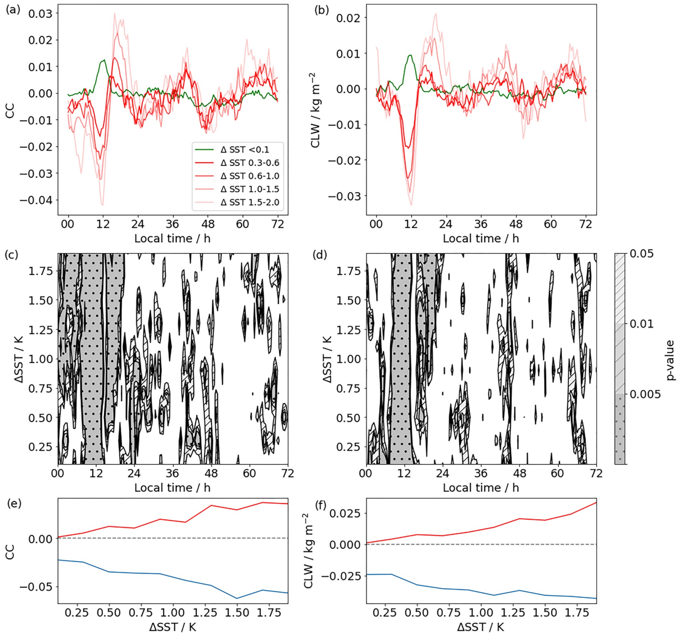
Figure 10. Time series of S_{+DWL} - S_{control} , t -test significance levels in bins of 0.1 K, and maximal (red) and minimal (blue) value of the deviation on the detection day for cloud cover (a, c, e) and cloud liquid water (b, d, f).
