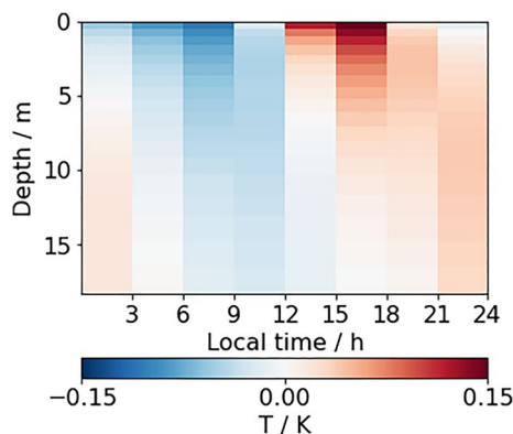
Figure 5. Sea water temperature (3 hr mean output) averaged over 3 days over the box 56.5^{\circ}\text{W}-59^{\circ}\text{W} and 12^{\circ}\text{N}-14.5^{\circ}\text{N} , time anomaly.
