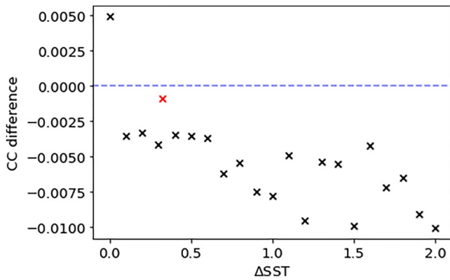
Figure 11. Diurnal mean cloud cover (CC) differences ( S_{+DWL} - S_{control} ) as a function of \Delta SST (black crosses). The red cross is the average CC difference against the average \Delta SST .
