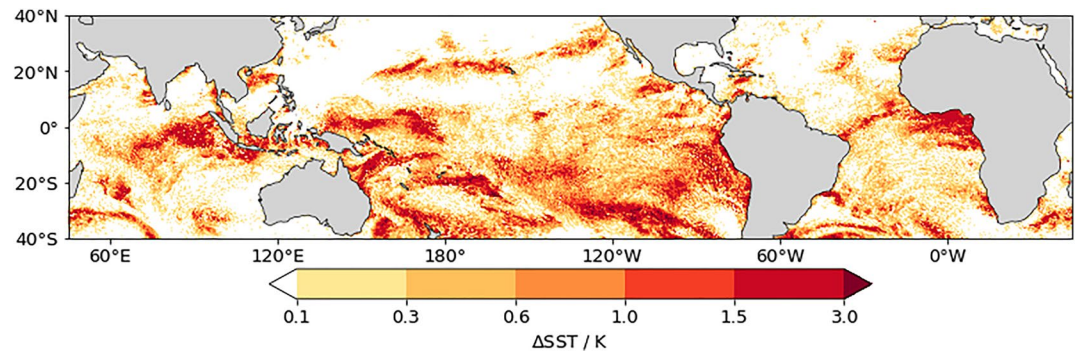
Figure B1. \Delta\text{SST} on detection day.
