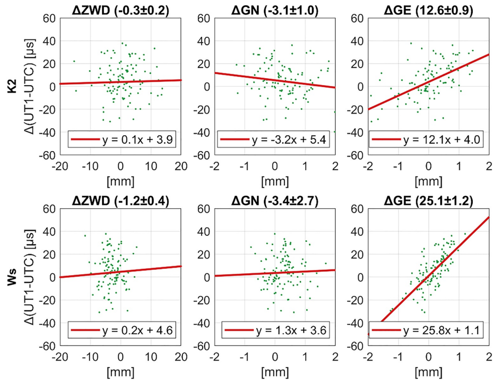
Figure 10. Linear regression analysis of Universal Time 1-Coordinate Universal Time (UT1-UTC) differences to tropospheric parameter differences between solution G0NT and G1AT for K2Wz (VGOS-2) sessions at KOKEE12M (upper panels) and WETTZ13S (lower panels) radio telescopes. Left to right: analysis of ZWD, north gradient, and east gradient. The simple regression analysis is shown as the red line in each subplot, and the multiple regression analysis coefficient and uncertainty for each tropospheric delay component are given in the title of the corresponding subplot.
