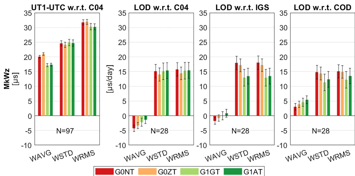
Figure 7. Results of Universal Time 1-Coordinate Universal Time (UT1-UTC) and Length of Day (LOD) for INT2 sessions between MK-VLBA and WETTZEILL radio telescopes. Left to right: UT1-UTC compared to 14C04, LOD compared to 14C04, LOD compared to International GNSS Service (IGS) product, and LOD compared to Center for Orbit Determination in Europe (COD) product. The uncertainty is given in the error bar.
