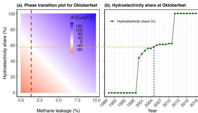
Figure 4. Left: phase transition diagram of hydropower shares in electricity generation versus methane leakage rates. It shows the difference in emissions (in tCO_2eq/TJ ) between electricity and natural gas as the energy source for heating and cooking at Oktoberfest. For positive values (blue shaded areas), the use of electricity leads to lower emissions compared to natural gas; for negative values (red shaded areas), the opposite is true. The red vertical dashed line represents the leakage rate of 1.4% measured at Oktoberfest, while the orange horizontal dashed line represents the associated share of renewable energy, where electricity is the more climate-friendly energy source compared to natural gas (58%). Right: share of renewable energies in electricity consumption at Oktoberfest. The dashed orange line shows that the share of renewable energies at Oktoberfest reached the break-even point from 2005 onwards, which means that electricity has been the more climate-friendly energy source than natural gas at the festival ever since.
