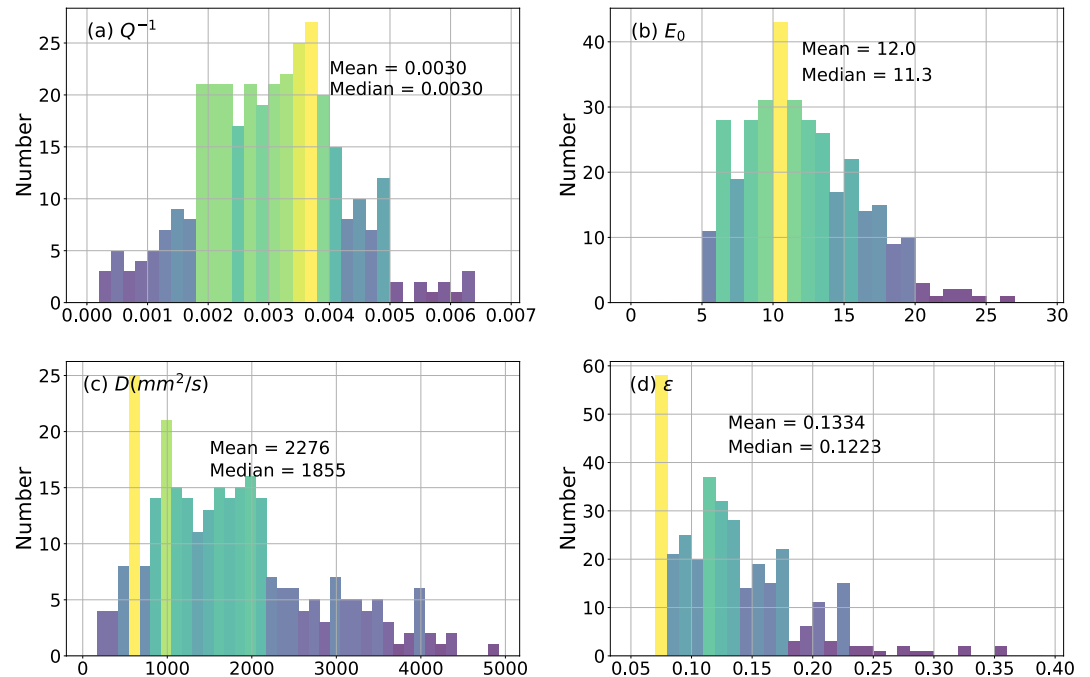
Figure 5. The statistics histograms of the parameters: (a) Q^{-1} , (b) E_0 , and (c) D estimated from all traces in the diffusion model, and (d) \epsilon calculated according to (c).
