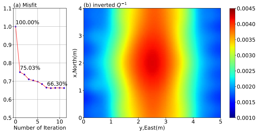
Figure 7. (a) The misfits of the later coda time window varied with iterations for the absorption inversion. (b) The inversion result of Q^{-1}(\mathbf{r}) after 11 iterations.
