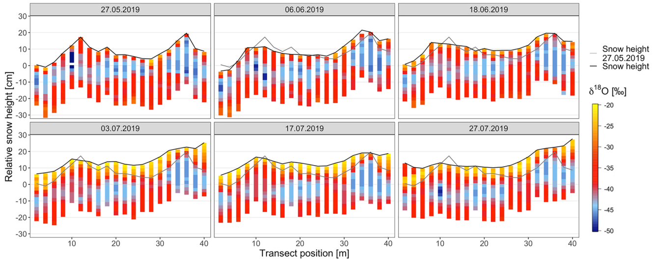
Figure 5. Two-dimensional view on the \delta^{18}\text{O} variability of each profile on a respective sampling day aligned with digital elevation model-derived snow height information. The black line indicates the relative snow height for each individual sampling day and the gray line the snow height of the first sampling day, that is, 27 May 2019. Transect position corresponds to the distance along the transect (Figures 1b and 1c).
