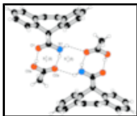
Fig. 2. The hydrogen bonded R_2^2(8) motifs of CYT-acetic acid joined in a centrosymmetric arrangement via an R_4^2(8) motif. Hydrogen bonds are shown as dashed lines.
