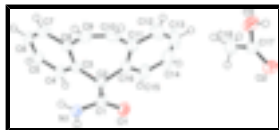
Fig. 1. The molecular structure of CYT acetic acid (1/1), showing 50% probability displacement ellipsoids.
