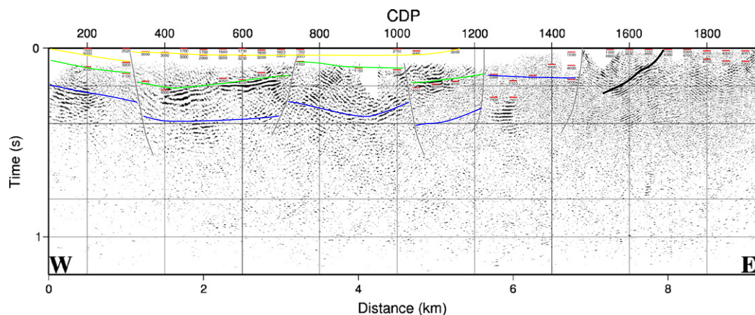
Fig. 10. Interpreted Mora profile. Times to refractors are plotted as short red lines at those CDP locations where a reasonable time–offset curve for the first arrivals could be picked. The velocity of the refracting interface is shown below each red line. Shown also are interpretations of the boundaries of the different geological units based on the reflection seismic images and the refraction interpretation. Yellow—base of the water saturated loose sediments, green—base of the Silurian, blue—base of the Ordovician, black—dolerite intrusion, gray—fault.
