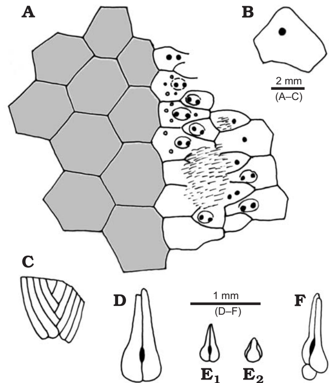
Fig. 5. Camera lucida drawings of test plating, tooth, and pedicellariae. A–E. Rhenechinus ibericus (Hauser and Landeta, 2007), Aguión Formation, Emsian, Lower Devonian, Arnao, Asturias, NW Spain. A. UO DGO-23000, adapical ambulacral and interambulacral (shaded) plating. B. UO DGO-23002, genital plate. C. UO DGO-23001, tip of oligolamellar tooth seen in axial view. D. UO DGO-23001, spinate tridentate pedicellaria. E. UO DGO-23000, two small tridentate pedicellariae (E 1 and E 2 ). F. Rhenechinus hopstaetteri Dehm, 1953, DBM.HS.285, spinate tridentate pedicellaria with basal element.
