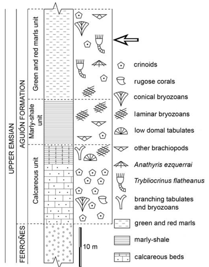
Fig. 2. Stratigraphical succession of the Aguión Formation at Arnao Platform showing lithological units, their faunal composition and types of communities. The level bearing echinoids is indicated by an arrow. From Arbizu et al. (1995).
