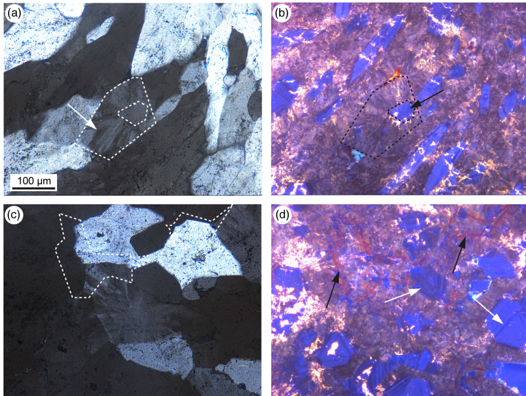
Figure 5. Photomicrographs (a, c) and CL images (b, d) of anhedrally to subhedral quartz grains exhibiting feathery textures. (a) Splintery or fibrous appearance of feathery textures, as indicated by the white arrow. The outer dashed line indicates the grain boundaries of one quartz grain, and the inner dashed line indicates a core with no feathery textures; X pol. (b) CL in which the patchy area of the feathery textures is shown by violet to reddish-brown colored with bright blue patches; the core is shown by intense blue luminescence. The patchy violet area makes up \sim 70 – 80 % of the image (exposure time: 22.2 s). (c) Photomicrograph of subhedral quartz grains locally showing feathery textures. The white dashed lines indicate intergranular zoning features (revealed in CL mode within d) X pol. (d) CL reveals red zoning features, which are indicated by black arrows. White arrows indicate growth zoning features within blue cores appearing in various shades of blue. The patchy violet area representing positions of feathery textures makes up \sim 60 – 75 % of the image (exposure time: 18.3 s) (non-oriented sample TY39X2).
