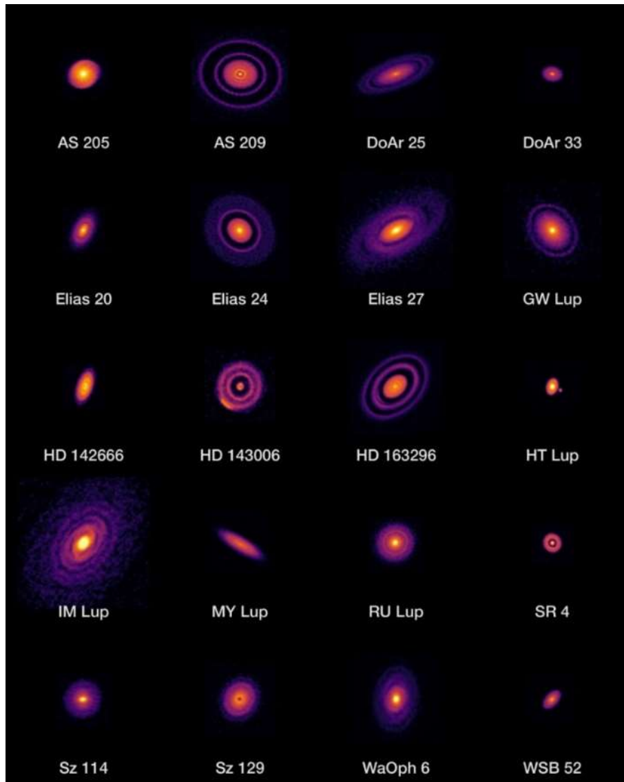
Figure 3. ALMA’s high-resolution images of nearby protoplanetary disks, which are the results of the Disk Substructures at High Angular Resolution Project (DSHARP). Credit: ALMA (ESO/NAOJ/NRAO), S. Andrews et al.; N. Lira
