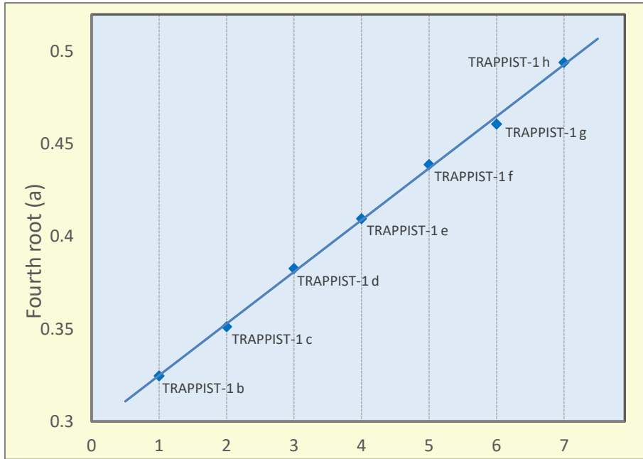
Figure 1. Distribution of planets in the ‘Trappist-1’ exoplanetary system
