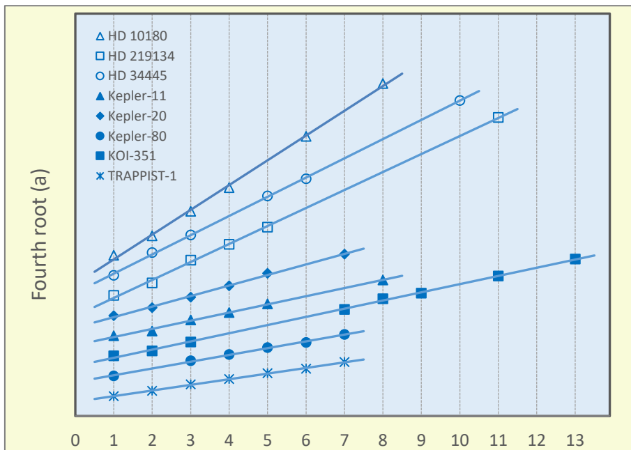
Figure 2. Distribution of planets in the exoplanetary system with six or more planets
