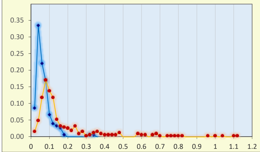
Figure 4. Normalised distribution of inclinations of the straight line (parameter A in equation y = Ax + B ) on the graph of V(a_n) vs. n for systems with two confirmed planets (orange) and for three and more confirmed planets (blue). The horizontal axis represents the values of parameter A , and the vertical axis represents the number of exosystems with inclinations in the intervals of 0.02 divided by the total number of exosystems (149 for systems with three and more confirmed planets and 303 for systems with two confirmed planets).
