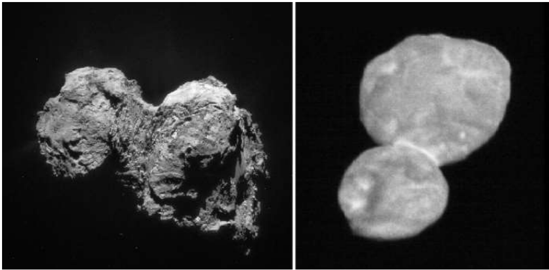
Figure 5. The images of Comet 67P/Churyumov-Gerasimenko (left, credit: ESA/Rosetta/NavCam) and Ultima Thule (right, credit: NASA/Johns Hopkins University Applied Physics Laboratory/Southwest Research Institute)
