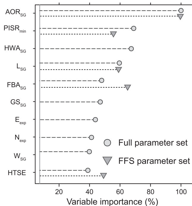
Figure 11. Relative scaled variable importance for random forests classification of landform segment activity using the full parameter set (points) and a reduced parameter set selected by forward feature selection (triangles). Variable importance given for 10 (of 16) most important parameters for the full parameter set and for 5 (of 9) from the reduced parameter set.
