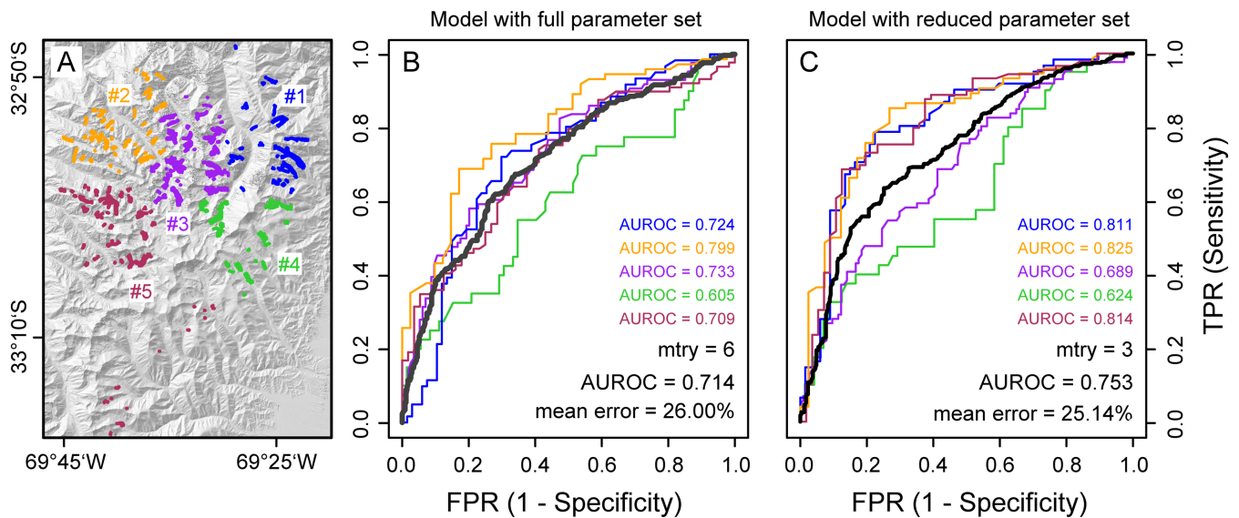
Figure 10. AUROC for landform segments using spatial cross-validation with five k -means clusters of the Cordón del Plata range. (A) Location map of n = 1020 landform segments, colour-coded by k -means spatial clusters: region #1 (blue), region #2 (orange), region #3 (purple), region #4 (green), region #5 (dark red). (B) AUROC for random forest classification using the full parameter set and (C) using the reduced parameter set. Curves in (B) and (C) are colour-coded according to the region left out (LLO-CV) for spatial cross-validation. Thick grey line gives mean AUROC of 125 model runs; TPR = true positive rate; FPR = false positive rate. [Colour figure can be viewed at wileyonlinelibrary.com]
