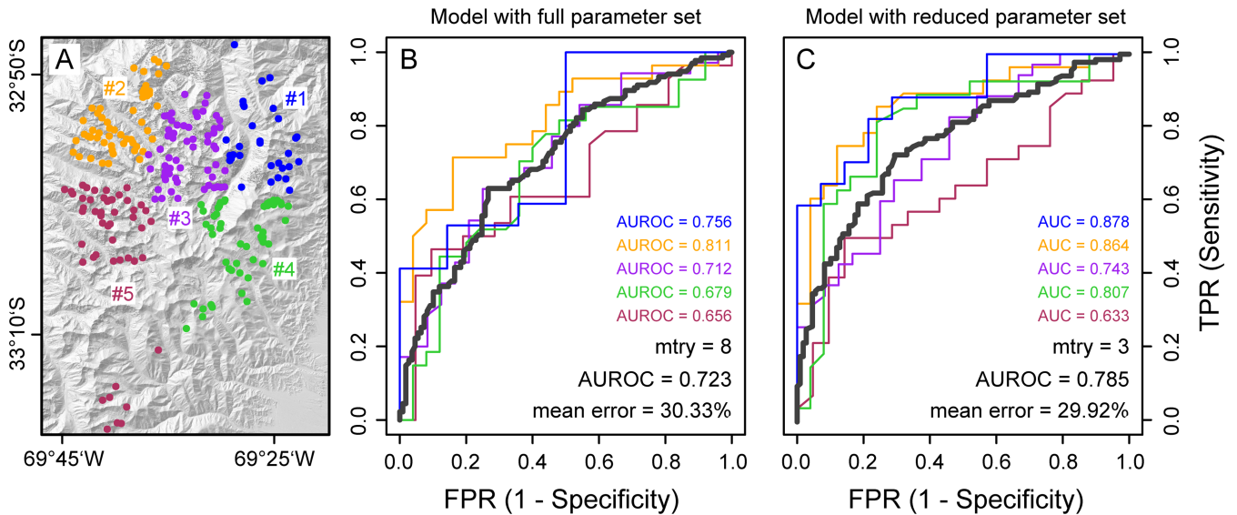
Figure 8. AUROC for landform polygons using spatial cross-validation with five k -means clusters of the Cordón del Plata range. (A) Location map of n = 244 rock glacier and ice-debris complex polygons, colour-coded by k -means spatial clusters: region #1 (blue), region #2 (orange), region #3 (purple), region #4 (green), region #5 (dark red). (B) AUROC for random forest classification using the full parameter set and (C) using the reduced parameter set. Curves in (B) and (C) are colour-coded according to the region left out for spatial cross-validation. Thick grey line gives mean AUROC of 125 model runs; TPR = true positive rate; FPR = false positive rate. [Colour figure can be viewed at wileyonlinelibrary.com ]
