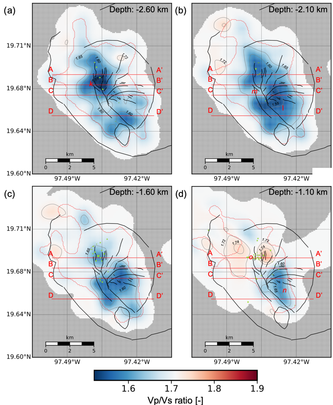
Figure 16. V_p/V_s structure at different depth levels. Panels (a)–(d) show depth slices for the resulting V_p/V_s model at -2.60 , -2.10 , -1.60 , and -1.10 km depths, respectively. Dashed red lines indicate the boundary at which spread values are less than or equal to 1.5 . Gray areas mark the regions where the DWS is less than or equal to 5 .
