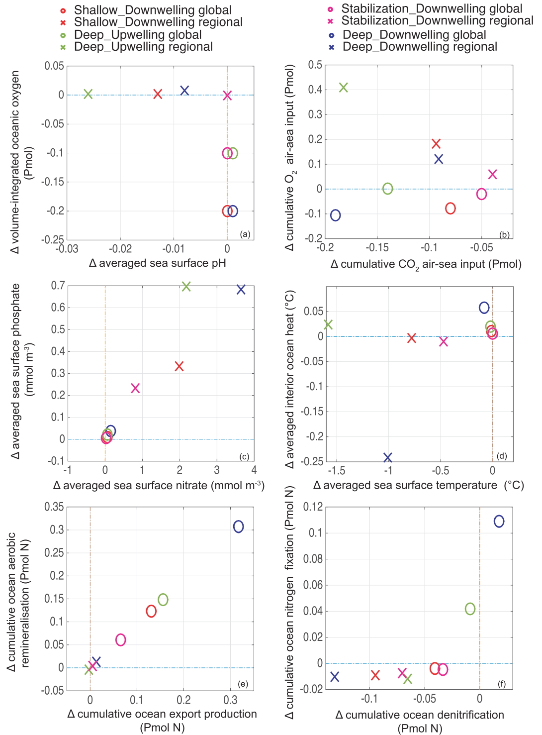
Figure 2. Differences between AD (AU) runs and the control run in year 2099. Globally averaged values are marked with circles while regionally (AD and AU implementation areas) averaged values are marked with crosses. The negative signs on panel b's axes refer to a gas flux from sea to air. Cumulative aerobic remineralization in panel (e) is computed below a depth of 130 m, the same depth used to compute export production.
