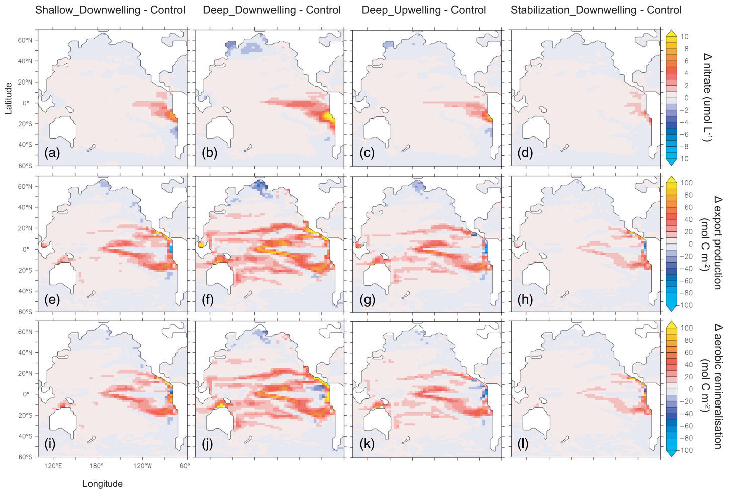
Figure 3. Differences in simulated sea surface nitrate for year 2099 of the Shallow_Downwelling (a), Deep_Downwelling (b), Deep_Upwelling (c), and Stabilization_Downwelling (d), respectively, with respect to the Control run; (e–h) the differences in cumulative (Years 2020–2099) export production of the respective model runs; (i–l) the differences for cumulative aerobic remineralization.
