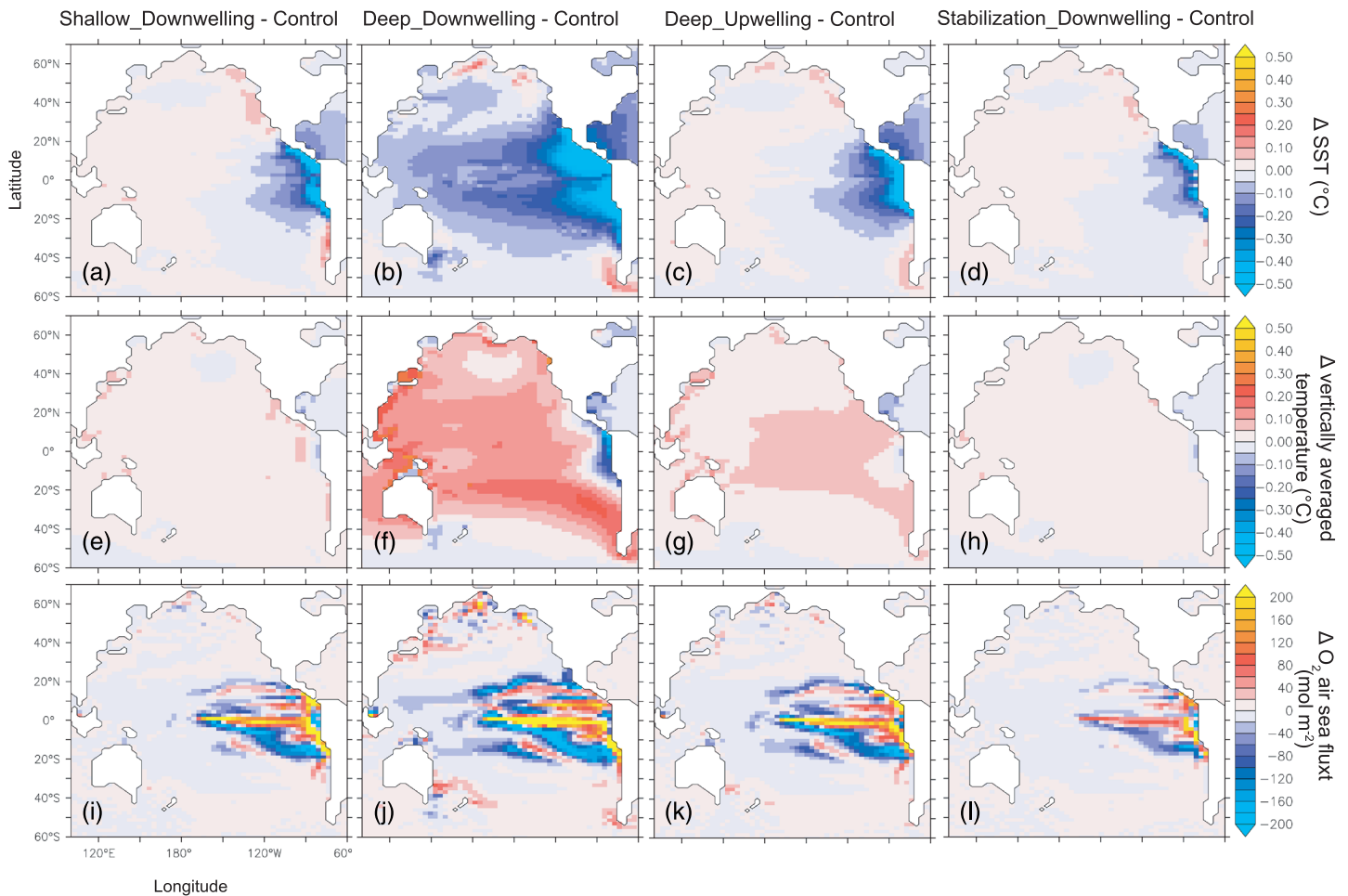
Figure 4. Referenced to the control run, changes of sea surface temperature (SST) simulated by run Shallow_Downwelling (a), Deep_Downwelling (b), Deep_Upwelling (c), and Stabilization_Downwelling (d), respectively, for year 2099; (e–h) following the same order, corresponding changes in ocean temperature vertically averaged over 50–1,600 m depth in year 2099; (i–l) changes in cumulative O_2 air-sea fluxes (positive values indicate an oxygen flux into the ocean) from year 2020 to 2099.
