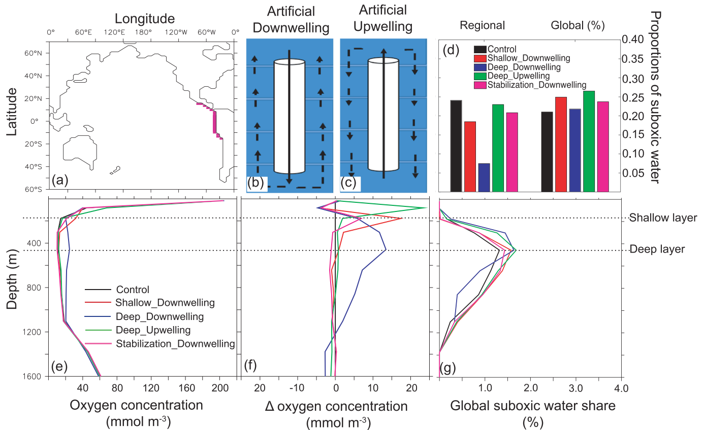
Figure 1. (a) Grid boxes along the west coast of Central and South America between 15.3°S and 15.3°N with AD (AU) implementation are marked violet (inside the dotted box). (b, c) Within each AD (AU) grid box, tracers were moved adiabatically from the sea surface layer to UVic’s Layers 3 (178 m depth) and 5 (457 m depth) for AD model run Shallow_Downwelling and Deep_Downwelling , respectively, while in the AU run ( Deep_Upwelling ) tracers were moved adiabatically from Layer 5 to the sea surface, during which a compensating upwelling (downwelling) flow was initiated in each AD (AU) grid box column to conserve volume. (d) Simulated volume percentage fraction of suboxic waters (oxygen concentration less than 5 μmol/L) with respect to the global ocean and volume fraction of regional suboxic waters with respect to the volume of the AD (AU) implementation area. (e) Vertical profile of area-averaged oxygen concentration in AD (AU) deployment regions. (f) Vertical profiles of AD (AU)-induced changes in oxygen concentration difference with respect to the control run in the deployment regions. (g) Vertical profile of the percentage of global suboxic area with respect to the global ocean area at the respective water depth. All results shown for model year 2099.
