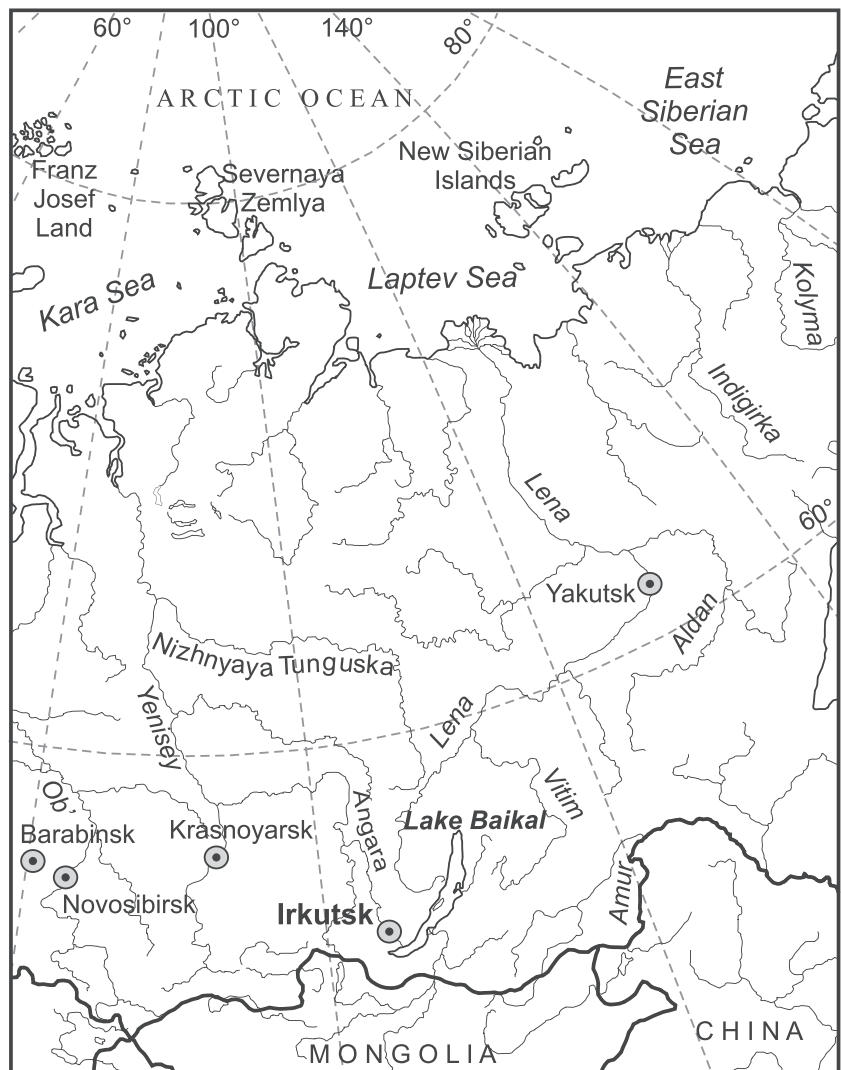
FIGURE 1 Schematic map of Eastern Siberia including the study site, the city of Irkutsk, situated close to Lake Baikal, and other points of interest
