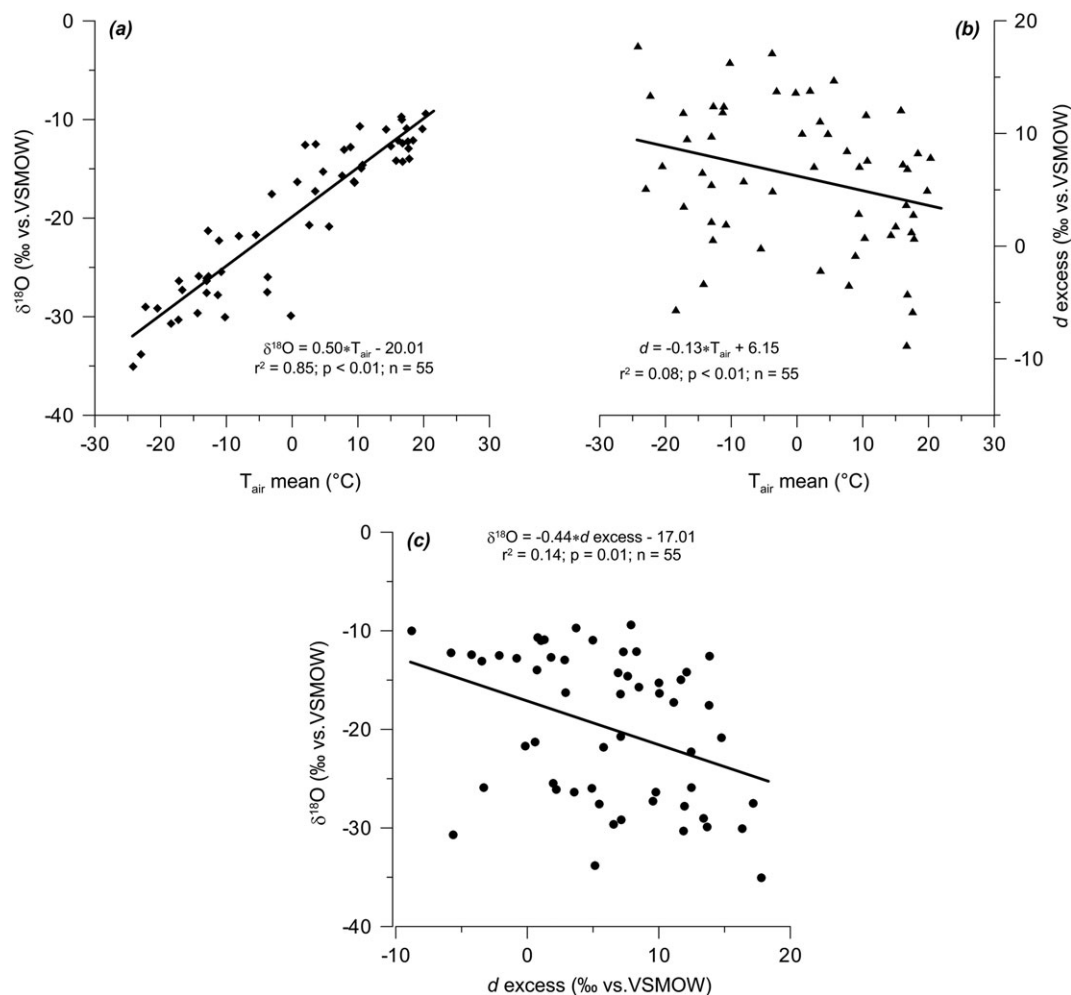
FIGURE 4 Correlations between (a) weighted mean monthly precipitation \delta^{18}\text{O} , (b) weighted mean monthly d excess and mean monthly temperature, (c) weighted mean monthly precipitation \delta^{18}\text{O} , and weighted mean monthly d excess
