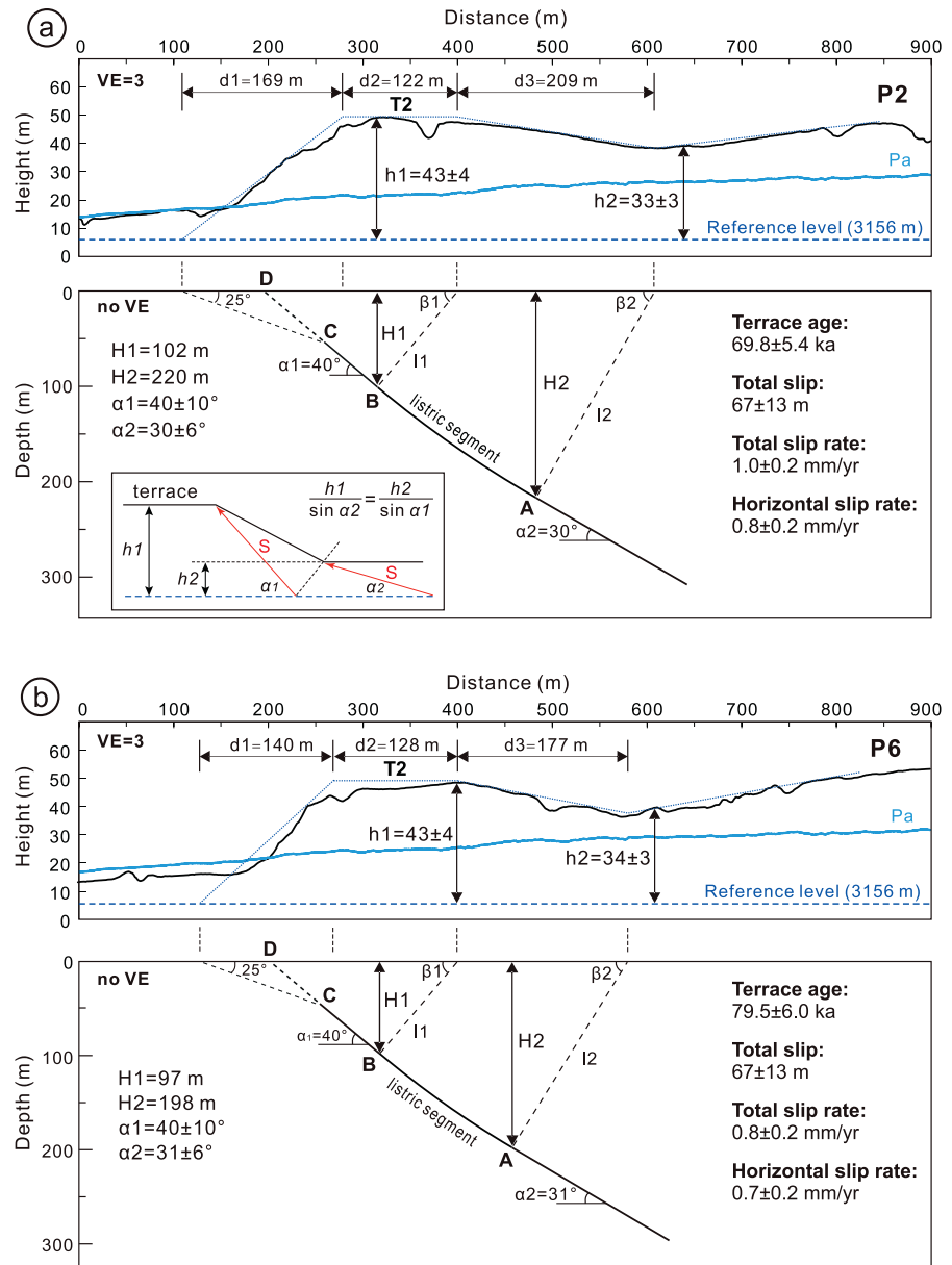
Figure 6. Topographic profiles P2 (a) and P6 (b) across the folded terrace T2 and modeled subsurface geometry of the thrust fault at depth. Both profiles were rotated by 2.5^\circ so that the reference level is horizontal. Parameters d_1 , d_2 , and d_3 are the horizontal length of the forelimb, the axial top, and the backlimb of the fold, whereas h_1 and h_2 are the terrace heights above the reference level at the axial top and just upstream of the backlimb. Points A and B delimit the listric fault segment, whereas H_1 and H_2 refer to the depth range of this segment. \alpha_1 and \alpha_2 are the dip angles of the planar fault segments above and below the listric fault segment. The planar fault dips 40^\circ between B and C but has a shallower dip of \sim 25^\circ close to the surface as revealed by paleoseismic trenches (Shao et al., 2017; for trench location see Figure 2). Inset shows the relation between terrace heights, fault slip S , and fault dip angles (cf. Hu et al., 2015).
