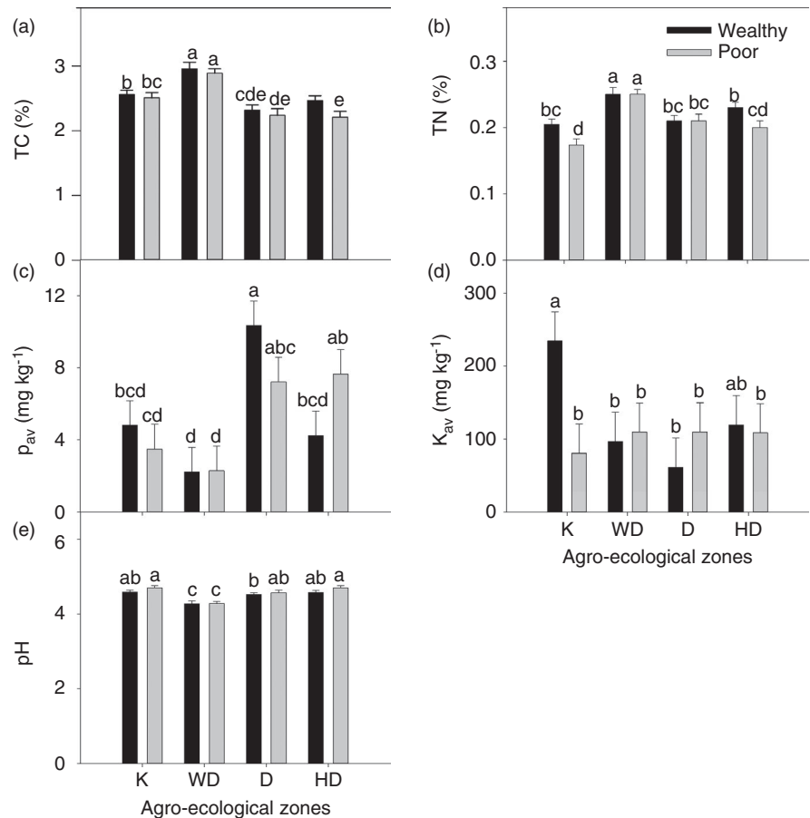
FIGURE 1 Soil chemical properties (a = total carbon [TC] [%]; b = total nitrogen [TN] [%]; c = available phosphorus [ P_{av} ] [ \text{mg kg}^{-1} ]; d = available potassium [ K_{av} ] [ \text{mg kg}^{-1} ]; e = soil pH) obtained from soils of fields of wealthy and poor farmers' fields across the four agro-ecological zones (K [Kola], WD [Weina-Dega], D [Dega], HD [High-Dega]). N = 215 for TC, TN and pH while 96 for ( P_{av} ) and ( K_{av} ). Bars with different letters on top of standard error indicate significant differences at p < 0.05
