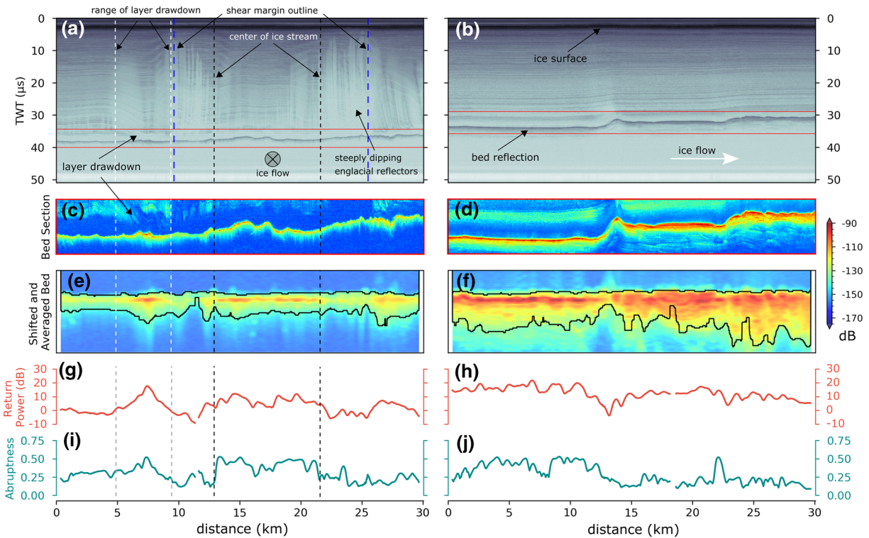
Figure 7. Two radar sections (two-way travel time (TWT) on the y-axis) and basal return echo properties from (a) an across-flow profile (location is indicated in Figures 6b and 6d with the blue outline) and (b) an along-flow profile (location is indicated in Figures 6a and 6c with the yellow outline). Panels c and d represent the analysis window of the ice-bed interface of the corresponding radargrams (indicated with the red lines in the radargrams) and their amplitude in dB. Panels e and f show the elevation-leveled basal reflectors and the corresponding BRP after along-track averaging. The black outline represents the window of integration for basal return power. The radargrams in panels a-f are neither corrected for spherical spreading nor englacial attenuation. Panels g and h show BRP corrected for spherical spreading as well as englacial attenuation (8 dB per km ice thickness) and (i) and (j) the waveform abruptness. The blue dashed lines in (a) show the position of the shear margins, the white dashed lines the region of layer drawdown outside of the shear margins and the black dashed lines the central part of the ice stream.
