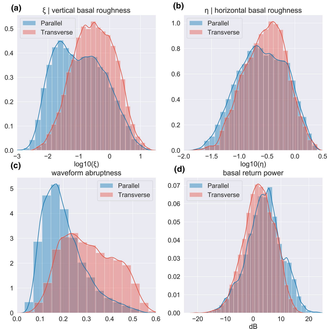
Figure 9. Histograms presenting the distribution of (a) vertical basal roughness, (b) horizontal basal roughness, (c) waveform abruptness, and (d) BRP for profiles oriented along- and across-flow for the location inside of the ice stream. The interpretation of anisotropy of BRP is limited due to the simple correction scheme for englacial attenuation. Blue bins represent along- and red bins across-flow profiles. The y-axis shows the kernel density estimation.
