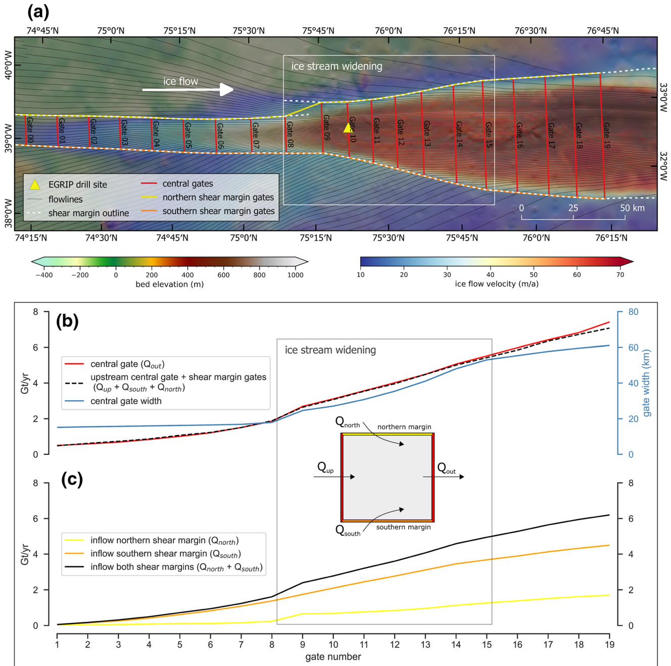
Figure 3. Flux gate analysis of the onset of the NEGIS. Panel (a) shows the position of central flux gates (red) and flux gates at the shear margins (yellow and orange, respectively). The location where the ice stream widens is marked with a white outline. Panel (b) shows the mass flux (in Gt/yr) through the central gates ( Q_{out} ; red line) in comparison to the sum of the respective upstream central gate ( Q_{up} ) and the corresponding shear margin gates ( Q_{south} + Q_{north} ; black dashed line). The blue line represents the width of the central gates. The cumulative mass flux through the northern and southern shear margin (as well as the sum of both) is shown in panel (c).
