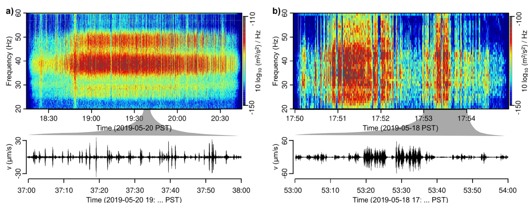
Figure 5. Seismic spectrograms and waveforms of additional signals recorded during the survey period. (a) A 2 h long activity period characterized by short-period 25–55 Hz pulses, most prominently recorded by station M12. (b) Example of recurring activity periods with similar properties as shown in (a) or Figure 2, recorded at station M11 1 . [Colour figure can be viewed at wileyonlinelibrary.com ]
