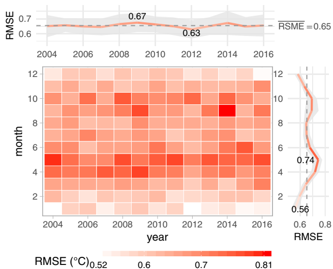
FIGURE 5 Root mean square error (RMSE) of the Stage 1 model using fivefold cross validation (CV5) for each month from 2004 to 2016. The model achieved an overall RMSE of 0.65^{\circ}\text{C} , with its annual and monthly means given in the top and right margins, respectively [Colour figure can be viewed at wileyonlinelibrary.com ]
