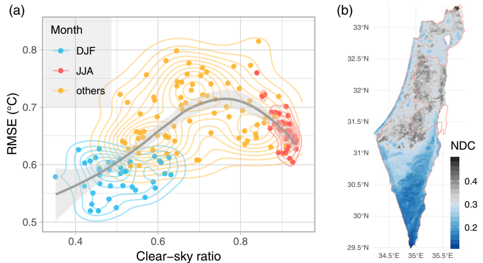
FIGURE 7 (a) Relationship between RMSE and clear-sky ratio (CSR) in the Stage 1 model for each month in the study period; and (b) the mean spatial pattern of the normalized difference cloudiness [NDC = (CSR_{JJA} - CSR_{DJF}) / (CSR_{JJA} + CSR_{DJF}) ] across Israel for all years. The NDC quantifies the fluctuation of clear-sky conditions between JJA (June–July–August, relatively cloudless) and DJF (December–January–February, the main rain season) [Colour figure can be viewed at wileyonlinelibrary.com ]
