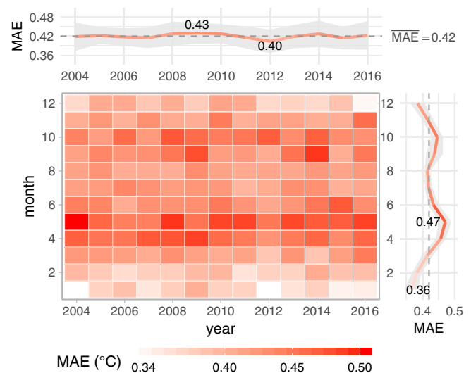
FIGURE 6 Mean absolute error (MAE) of the Stage 1 model using fivefold cross validation (CV5) for each month from 2004 to 2016. The model achieved an overall MAE of 0.42^{\circ}\text{C} , with its annual and monthly means given in the top and right margins, respectively [Colour figure can be viewed at wileyonlinelibrary.com ]
