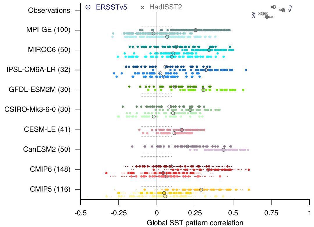
Figure 3. Global pattern correlation of each realization from CMIP5, CMIP6, the single-model large ensembles, and two observational estimates compared to the observational estimate COBE-SST2. The four rows (bottom to top) for each ensemble correspond to the early warming, the early hiatus, the recent warming, and the recent hiatus. Gray circles show the ensemble mean, and the dashed horizontal lines indicate missing data in the simulations. For CMIP6 and CMIP5, the larger filled dots show the first ensemble member of each model and the small dots all other ensemble members.
