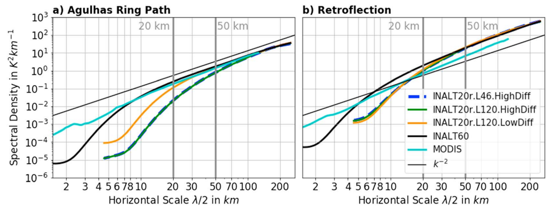
Figure 7. The 2012–2017 time-mean sea surface temperature spectra for the Agulhas ring path (a) and the retroreflection (b). Both subregions are marked in Figure 6. The horizontal scale is identified as half the wavelength \lambda .
