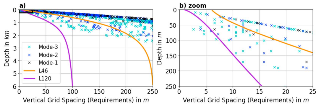
Figure 4. The vertical grid spacing as a function of depth for the 46 vertical levels (L46) and the 120 vertical levels (L120). Crosses show the requirements on the vertical grid spacing to resolve the first, second, and third baroclinic mode as derived by Stewart et al. (2017) from CTD measurements at the locations shown in Figure 1c. The right panel shows a zoom into the near-surface box marked in the left panel.
