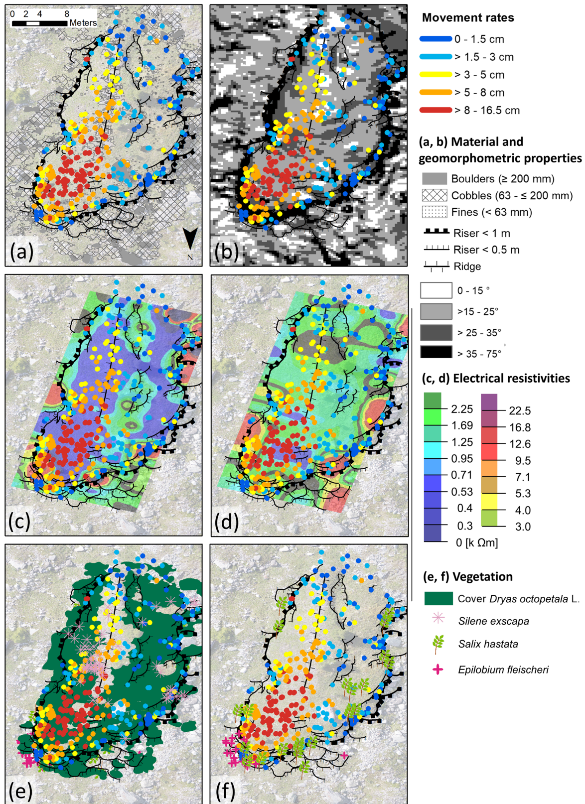
FIGURE 3 Geomorphometric, material and vegetation properties in relation to solifluction displacement (2014–2017) derived from unmanned aerial vehicle-based mapping. (a) Geomorphologic map with landform elements and material properties in relation to displacement patterns. (b) Slope gradient map in relation to displacement patterns. Result from 3D ERT in relation to displacement patterns for (c) depth of 0–0.75 m and (d) depth of 0.75–1.5 m. Simplified vegetation map for (e) lobe tread and ridge feature as well as (f) lobe risers. See Eichel et al. 8 for more detailed vegetation maps [Colour figure can be viewed at wileyonlinelibrary.com ]
