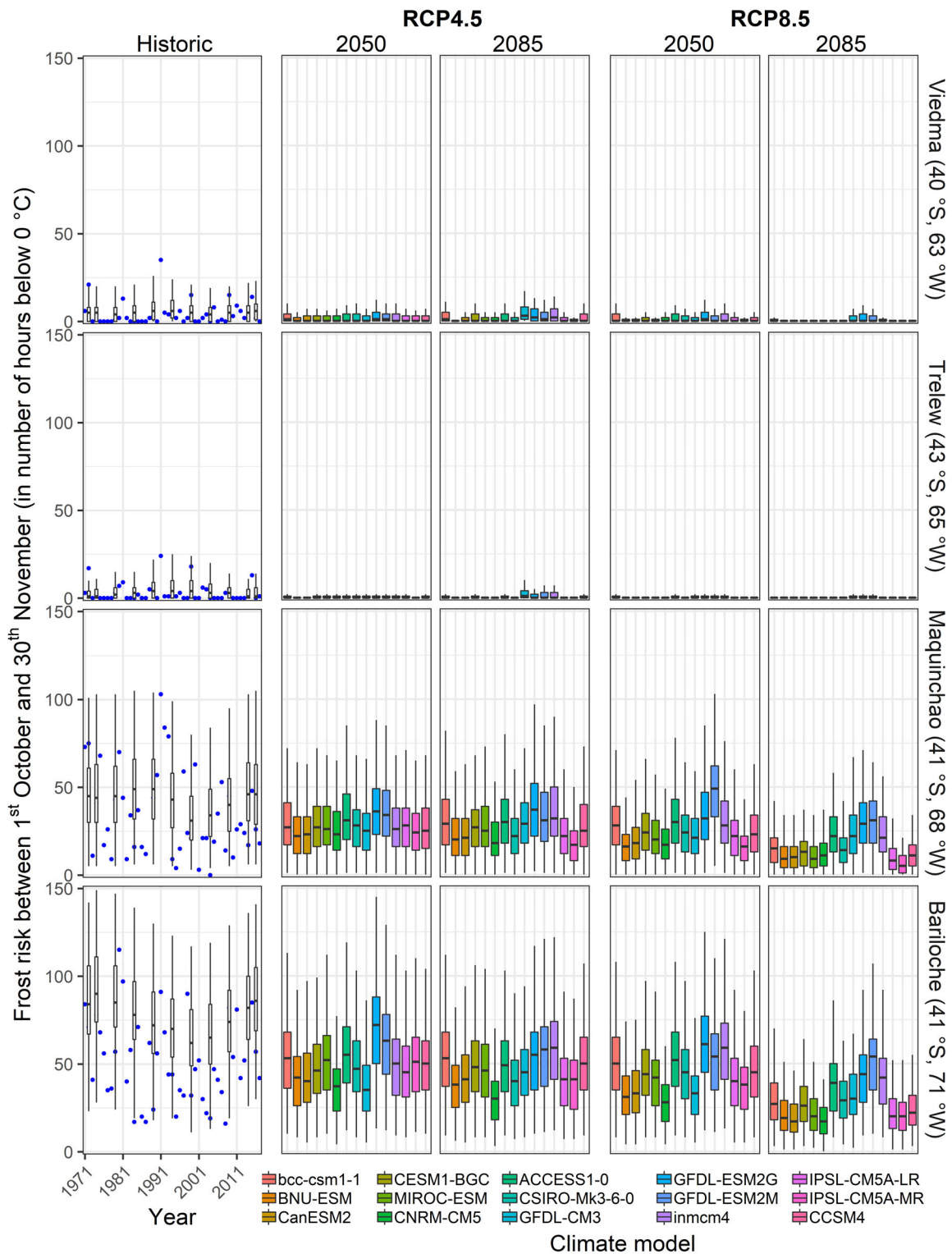
FIGURE 6 Historic and projected future number of spring frost occurrences (number of hours below 0°C) between 1st of October and 30th of November in four sites of Argentinean Patagonia (Viedma, Trelew, Maquinchao and Bariloche). In the left hand “Historic” panels, dots represent the actual spring frost computed from the historic record and boxplots represent the frost computed for the simulated historic weather scenarios. In future scenarios (RCP4.5 and RCP8.5 panels), boxplots represent the distribution forecasts according to the climate models. The left-to-right order for boxplots in future panels refers to the top-to-bottom order in climate model legend [Colour figure can be viewed at wileyonlinelibrary.com ]
