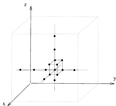
Figure 15 A chain subgraph knot of k \cdot K_{\text{pcu}} .
