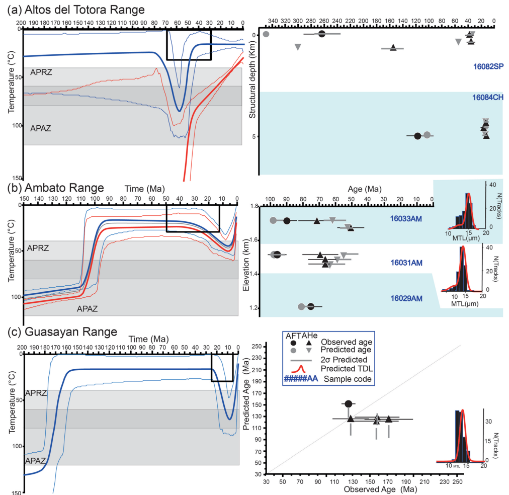
Figure 6. Thermal history expected models from the (a) Altos del Totora, (b) Ambato, and (c) Guasayan ranges. See Figure 4 for a detailed caption.
