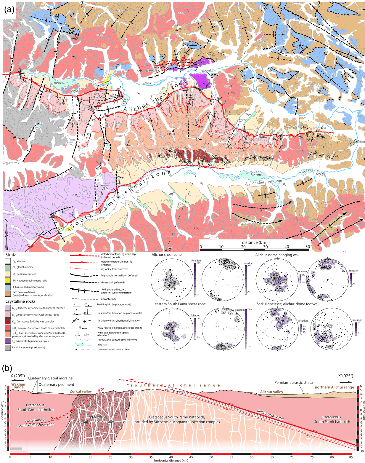
Figure 2. (a) Geologic map of the Alichur dome, based on Yushin et al. (1964), Stübner, Ratschbacher, Rutte, et al. (2013), and our mapping. 500 m contour interval. Stereonets show compiled structural data from all stations for all major tectonic domains. (b) Strike-normal cross section transecting the Alichur dome. Location of cross section shown in Figure 2a.
