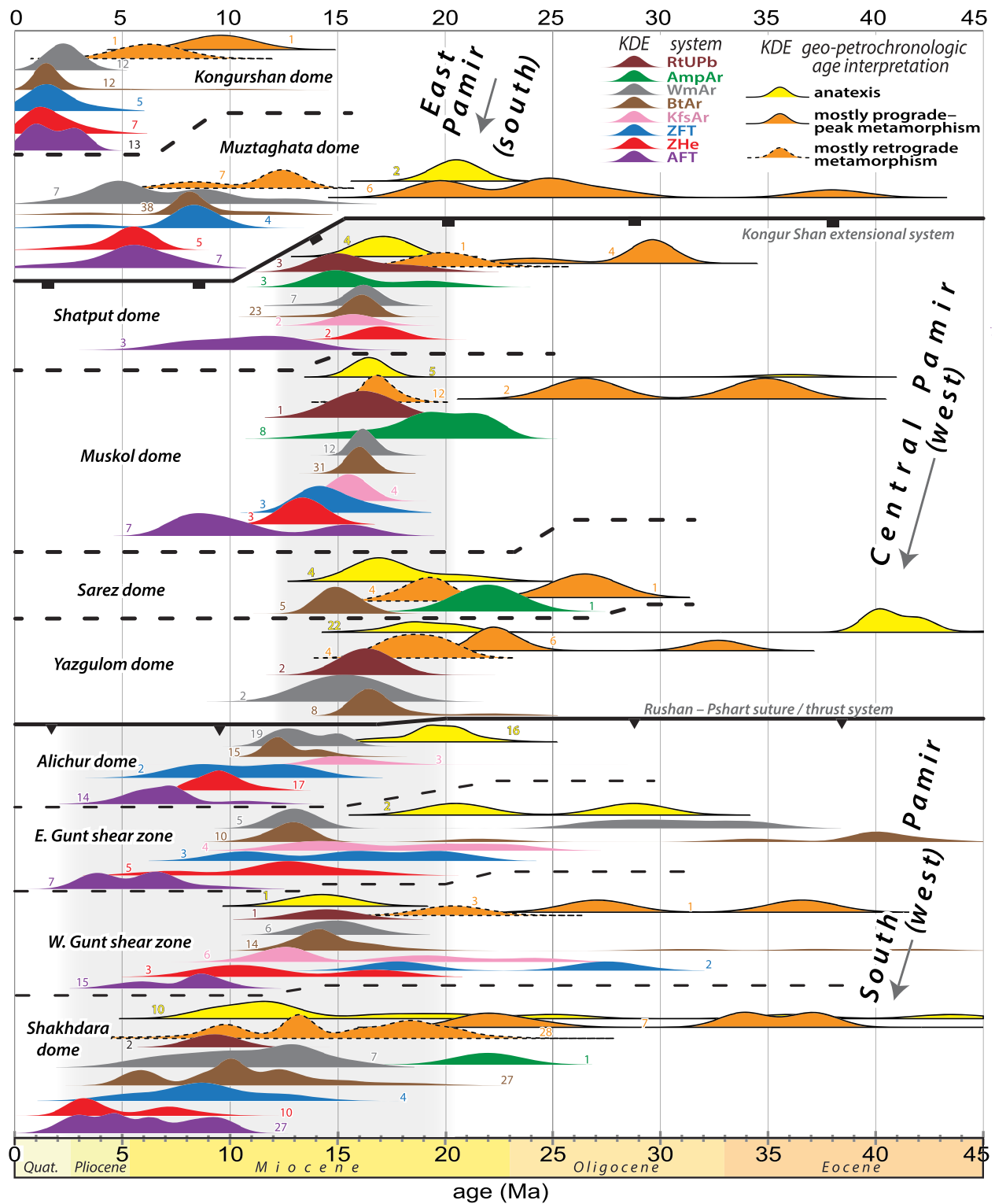
Figure 5. Compiled kernel density estimates (KDEs) of geo-petro-thermochronologic ages for bedrock samples from the Pamir gneiss domes (Cai et al., 2017; Cao, Wang, et al., 2013; Chapman, Robinson, et al., 2018; Chapman, Scoggin, et al., 2018; Hacker et al., 2017; Hubbard et al., 1999; Robinson et al., 2004; Robinson et al., 2007; Rutte, Ratschbacher, Khan, et al., 2017; Schmidt et al., 2011; Stearns et al., 2013; Stearns et al., 2015; Stübner, Ratschbacher, Weise, et al., 2013). Shaded vertical bands highlight the timing of ~N-S extensional gneiss-dome exhumation in the Central and South Pamir; the East Pamir is not addressed. The eastern and western Gunt shear zone are included for comparison to the Alichur and Shakhdara domes. KDEs (adaptive bandwidth = 1 Myr) plotted using DensityPlotter 7.3 (Vermeesch, 2012). U/Pb mixed ages plotted using average of minimum and maximum ages and setting 2\sigma to the mixed-age range.
