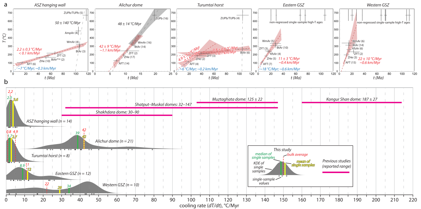
Figure 6. (a) Bulk-average cooling-rate estimates through medians of pooled cooling ages and their closure temperatures. Error crosses indicate \pm 2\sigma_M for pooled cooling ages and \pm 2\sigma = 10\% for pooled closure temperatures for each chronometer. Red error envelopes and lines indicate post-magmatic conductive cooling; dashed blue lines indicate exhumation-related cooling through intermediate–low temperatures; gray error envelopes and lines indicate exhumation-related cooling through intermediate–low temperatures; gray error envelopes and lines indicate post-magmatic conductive cooling; dashed blue lines indicate exhumation-related cooling through intermediate–low temperatures; gray error envelopes and lines indicate exhumation-related cooling through intermediate–low temperatures. (b) Kernel density estimators (KDEs) of single-sample cooling rates for the ASZ hanging wall, Alichur dome, Turumtai horst, eastern and western Gunt shear zone (GSZ). Medians and means of single samples indicated in red and blue; bulk-average estimates (regressions through medians of pooled cooling ages) shown in yellow for comparison. Previously reported cooling-rate ranges for other Pamir gneiss domes shown for comparison (Cao, Wang, et al., 2013; Hacker et al., 2017; Rutte, Ratschbacher, Khan, et al., 2017; Stübner, Ratschbacher, Weise, et al., 2013). KDEs plotted use 3 °C/Myr adaptive bandwidth with DensityPlotter 7.3 software (Vermeesch, 2012).
