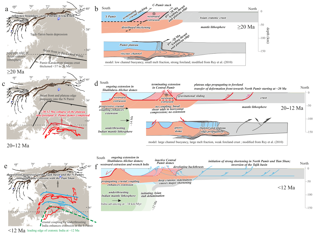
Figure 8. Geodynamic model for the evolution of the Central and South Pamir, refined from Rutte, Ratschbacher, Khan, et al. (2017). (a and b) The \geq 37 –20 Ma development was characterized by crustal thickening resulting in up to 90 km-thick crust, the formation of the Pamir plateau, and the generation of a viscous channel beneath the plateau. Low channel buoyancy, a small melt fraction, and a strong foreland upper crust favored foreland-directed channel-flow extrusion beneath the plateau (Rey et al., 2010). The leading edge of the Pamir plateau was located along the Central Pamir. (c and d) Indian slab breakoff at 25–20 Ma changed the channel properties. The heat input and the regional migmatization documented in the exposed South Pamir lower–middle crust inhibited channel flow, favoring core-complex formation in the Pamir plateau (the Central and South Pamir gneiss domes). The collapse of the Pamir crust from ~21 Ma onward relocated the deformation front from the Central Pamir to the North Pamir. Earlier termination of ~21 Ma extension in the Central Pamir with respect to the South Pamir is attributed to its position at the former northern periphery of the Pamir plateau, where the thick, hot crust was transitioned northward into the cold, thin Tajik–Tarim foreland. At ~12 Ma, the formation of the Central Pamir gneiss domes was completed. After the 25- to 20-Ma break-off of Greater Indian lithosphere, the India–Asia convergence was characterized by underthrusting (Kufner et al., 2016). The resulting strong coupling between underthrusting Indian lower crust and overlying Asian crust (Copley et al., 2011; Liu & Yang, 2003) enhanced ~N–S extension in the underthrust South Pamir (where it continued until ~4–2 Ma) and inhibited ~N–S extension in the non-underthrust Central Pamir (where it ceased by ~12 Ma). (e and f) Greater ~N–S extension in the Shakhhdara dome than in the Alichur dome reflects a triangular geometry of the underthrusting Indian promontory, which facilitated stronger coupling beneath the western Pamir than the eastern Pamir. The onset of out-of-sequence thrust-wrenching in the Central Pamir and the northern South Pamir by ~12 Ma reflects the initiation of northward delamination and roll-back of Asian lithosphere by northward bulldozing Indian lithosphere (Kufner et al., 2016). The shear zones in the Central Pamir and northern South Pamir have dominantly top-N kinematics, whereas the exhumation of the Shakhhdara dome occurred along the top-SSE South Pamir shear zone (SPSZ). Rey et al.’s (2010) conceptual model of gravitational-collapse-driven plateau growth attributes the Central Pamir top-N collapse to mass transfer by gravitational sliding of the plateau edge onto the foreland (see panel d). The SPSZ constitutes an antithetic shear zone in the orogenic hinterland that accommodated the formation of a large metamorphic-core complex, exposing a weak, formerly northward-flowing lower–middle-crustal channel. The upper crust south of the SPSZ was relatively stationary, whereas the Shakhhdara-dome crust spread northward and upward beneath it.
