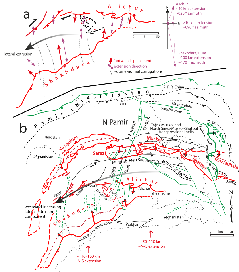
Figure 7. (a) Structural-kinematic framework of the Shakhdara–Alichur gneiss-dome complex highlighting dominant ~N–S extension along detachment faults (red) and minor ~E–W extension and dextral wrenching along secondary structures (black). Footwall displacement vectors and extension directions along the detachments are grossly scaled for the variable along-strike displacement/strain of the gneiss-dome complex. Azimuthal divergence in displacement/strain is highlighted in the vector diagram to the right, employing maximum values for extension. The Turumtai horst is a low-strain relay bridge between the Shakhdara and Alichur domes and accommodates extension at the eastern terminus of the Gunt shear zone (GSZ). The segmented GSZ, likely with mostly normal displacements in its early history, is one of several dextral shear zones mapped from the Wakhan of Afghanistan in the south to the Central Pamir in the north (Rutte, Ratschbacher, Schneider, et al., 2017; Stübner, Ratschbacher, Rutte, et al., 2013) (see panel b). The dome-normal corrugations are mega-boudins indicating minor ~E–W extension. Relative to the weakly deformed crust of the eastern South Pamir (east of the Alichur dome), the boudinage and wrenching accommodate a westward-increasing flow component—westward lateral extrusion—of the Pamir plateau crust, secondary to the dominant northward material flow. (b) The Neogene gneiss-dome system of the Central and South Pamir (in red) and the fault network of the neotectonic deformation field (in green). Faults in black have unknown timing or formed at an intermediate stage, and have overwhelmingly dextral-transpressive kinematics. Major fault zones discussed in the text are named. Cumulative ~N–S extension across the gneiss domes (bottom) is larger in the west (Shakhdara–Yazgulom transect) than east (Alichur–Muskol transect). Whereas a westward-increasing lateral-extrusion component for the neotectonic deformation field is given by the ~N-striking normal-fault systems and dextral strike-slip component along the Pamir thrust system, that for the Neogene deformation field is traced by the mega-boudin structure of the domes and the distributed wrench belts in the Central and South Pamir.
