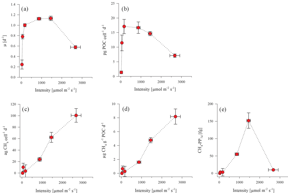
Figure 3. Relationship between light intensity and growth rate (a), POC production rate (b), cellular (c), and POC normalized \text{CH}_4 production rate (d) and \text{CH}_4 -PP e of E. huxleyi . Values are the mean of four replicated culture experiments with SD.
