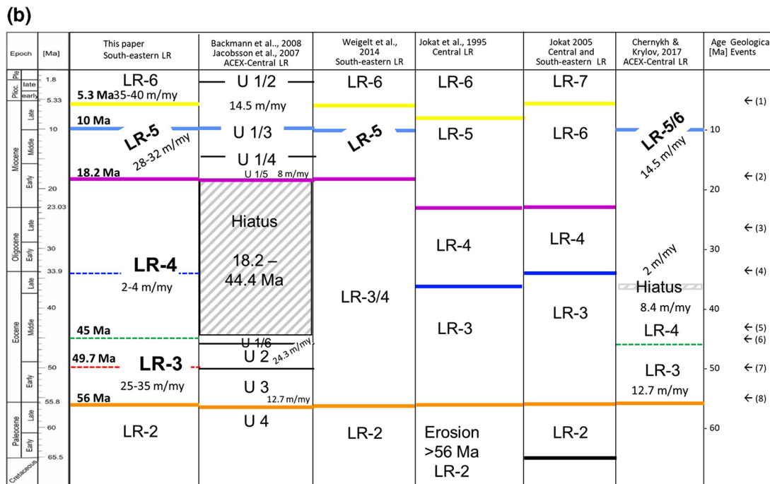
Figure 2. (a) Compilation of stratigraphic models of the southeastern Amundsen Basin and (b) extrapolated to the southeastern crest of the Lomonosov Ridge. Time scale after Gibbard et al. (2010). Colored bars mark major interfaces, sedimentation rates are given in m/Myr. Arrows with numbers mark the geological events: (1) Large-Scale Glaciation of Northern Hemisphere (Zachos et al., 2001); (2) deep-water connection through Fram Strait to North Atlantic, modern current system in the Arctic Basin (Jakobsson et al., 2007); (3a-b) widening and deepening of the Fram Strait and periodic incursions of North Atlantic waters (Jakobsson et al., 2007); (4) change in relative plate motion and initial opening of Fram Strait; (5) “Azolla” Fresh Water Event (Brinkhuis et al., 2006); (6) subsidence of LR well below sea level (Jokat et al., 1995); (7) LR in shallow water depth (Jokat et al., 1995); and (8) break up of LR and onset of seafloor spreading (Karasik, 1968; Vogt et al., 1979). AB, Amundsen Basin; LR, Lomonosov Ridge.
