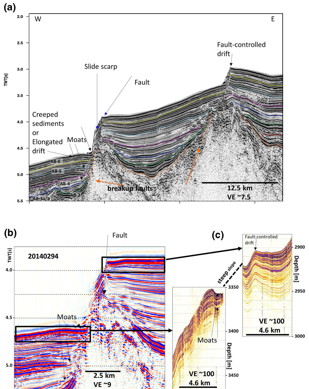
Figure 8. (a) Ridge-slope terraces on enlarged section of seismic line AWI-20140294 (for location see Figure 1a, and Figures 5 and 6). Old rifting structures are marked in orange. Yellow reflector = early Pliocene, light blue reflector = late Miocene, pink reflector = Top Oligocene. (b) Ridge-slope terraces on seismic line AWI-20140294. The water column is not muted to emphasize steep slopes. Black frame shows location of Parasound sections. (c) Parasound section, the profile is interrupted because the slope is steeper than 4^\circ and reflection signals are scattered.
