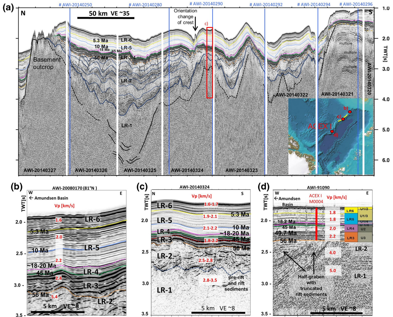
Figure 3. (a) Seismic lines AWI-20140320 to AWI-20140327 along the Lomonosov Ridge (for location see Figure 1a). Early Pliocene (yellow), top of HARS (High Amplitude Reflector Sequence) = Top Oligocene (pink), early Eocene (orange), basement (black). Blue bars: Intersections with seismic lines across the Ridge and corresponding line numbers. The index map shows the location of the analyzed profiles (yellow line) and subfigures (red dots). (b) Classification of units, corresponding interval-velocities in km/s (red number), and marker horizons, (c) the southeastern end of the LR, and (d) at the location of ACEX-I with the incorporated seismostratigraphic model after Backmann et al. (2008).
