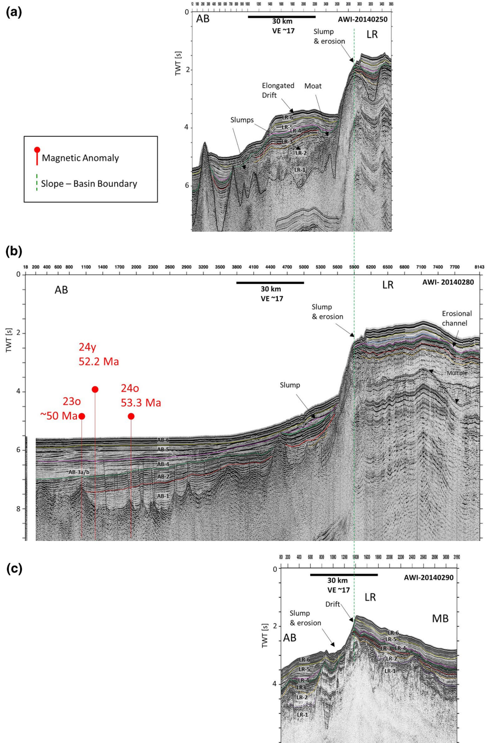
Figure 6. Compilation of lines north of 83° across the Lomonosov Ridge, slope, and adjacent Amundsen and Makarov Basins (for location see Figure 1a). AB, Amundsen Basin; LR, Lomonosov Ridge; MB, Makarov Basin. All lines are in same scale and aligned at the slope-basin boundary. Black frames show the location of discussed profile sections. Red marker: cross-points with magnetic anomalies after Chernykh & Krylov (2011), and Gaina et al. (2011). Marker horizons are: Early Pliocene (~5.3 Ma, yellow), late Miocene (~10 Ma, light blue), Top Oligocene (18–20 Ma, pink), Top Eocene (~34 Ma, blue), middle Eocene (~45–47 Ma, green), early Eocene (~49–50 Ma, red), Base Eocene (~56 Ma, orange), acoustic basement (black).
