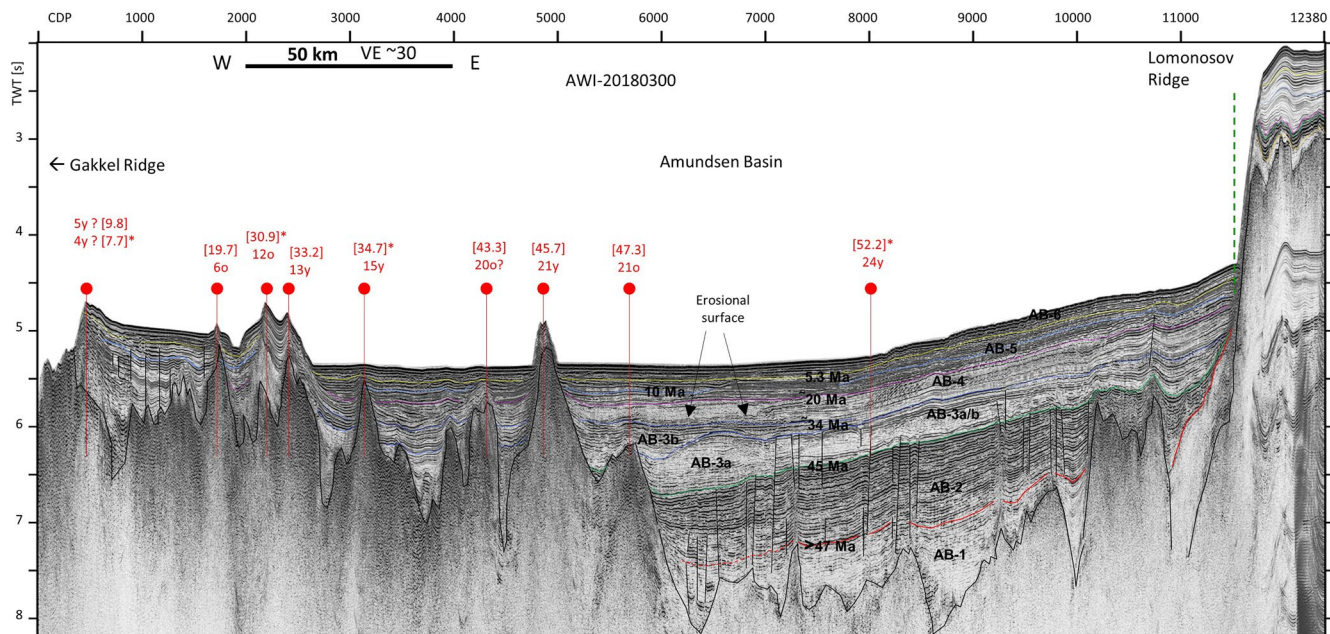
Figure 4. Seismic line AWI-20180300 across the Amundsen Basin (for location see Figure 1a) showing units AB-1 to AB-6 (black). Cross-points with magnetic anomalies (red markers) and magnetic chrons (red numbers). Corresponding age (in brackets) in Ma after Ogg (2012); and * after Chernykh and Krylov (2011) and Gaina et al. (2011). Marker horizons: Early Pliocene (yellow, 5.3 Ma), late Miocene (light blue, 10 Ma), Top Oligocene/Base Miocene (pink, 20 Ma), base Oligocene (dark blue, 34 Ma), middle Eocene (green, 45–47 Ma), early Eocene (red, 49–50 Ma), acoustic basement (black, <56 Ma). Slope-basin boundary (green dashed line).
